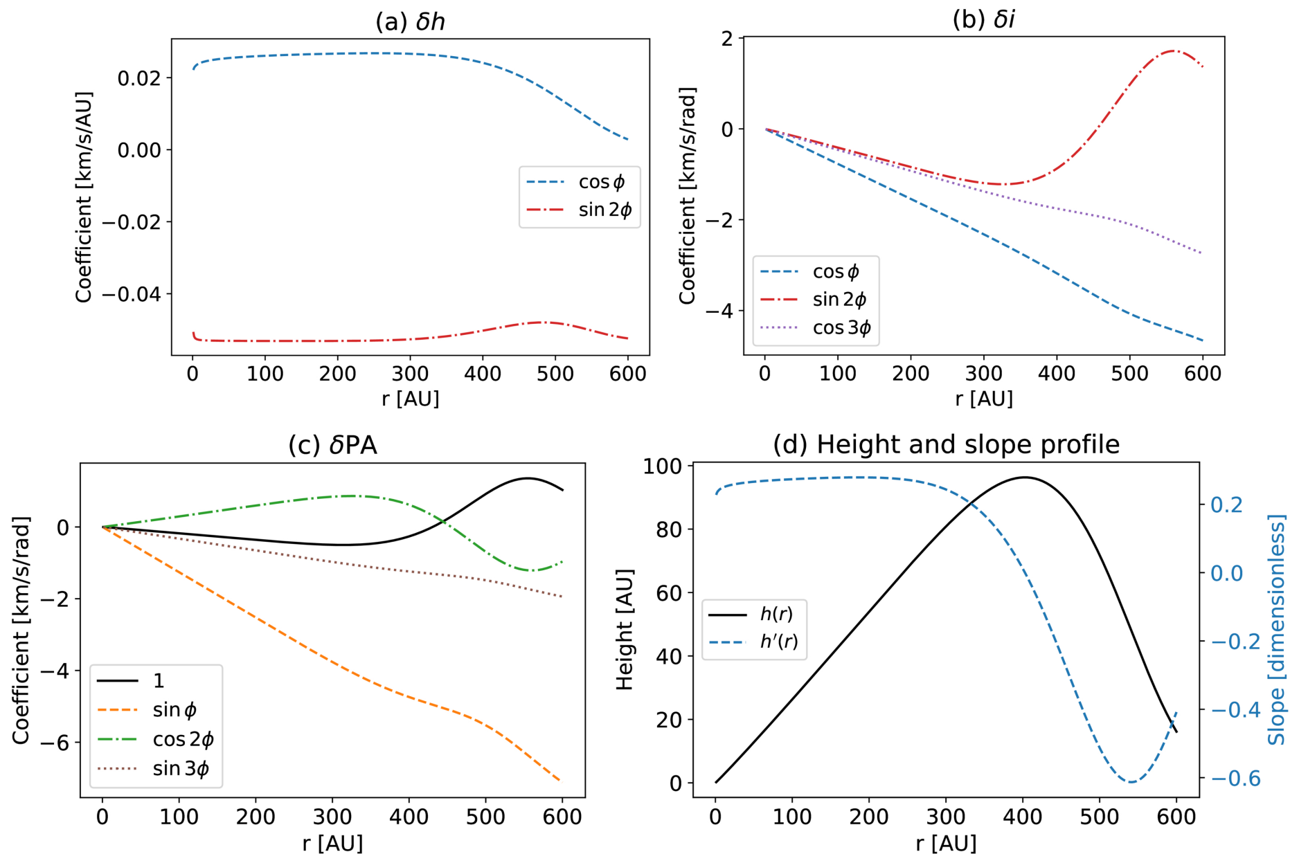
Figure 4. from Masataka Aizawa and Ryuta Orihara 2026 Astron. J. 171 doi:10.3847/1538-3881/ae1a75 https://dx.doi.org/10.3847/1538-3881/ae1a75 © 2025. The Author(s). Published by the American Astronomical Society.
