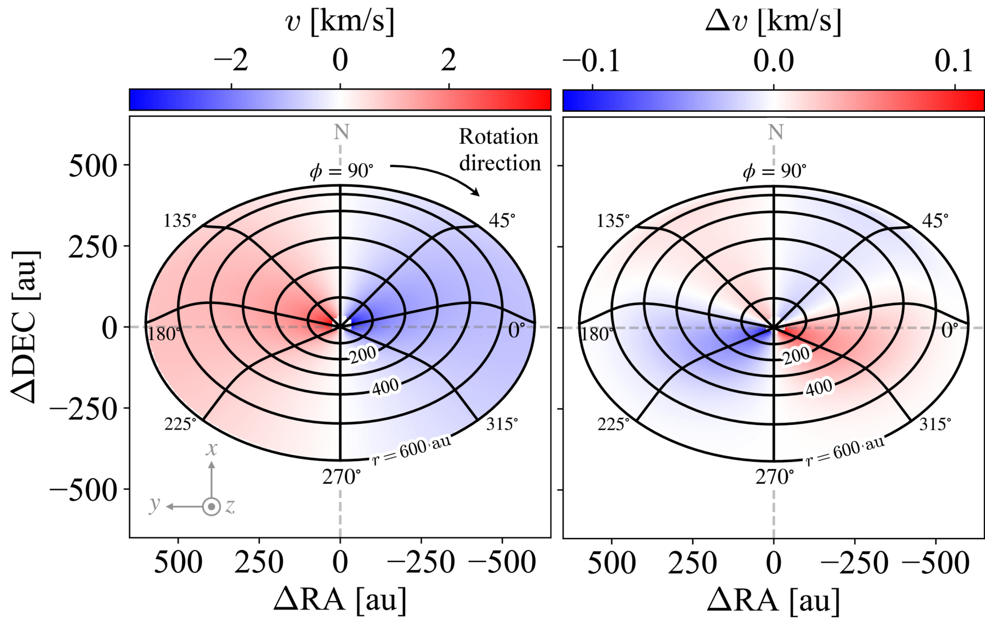
Figure 2. from Masataka Aizawa and Ryuta Orihara 2026 Astron. J. 171 doi:10.3847/1538-3881/ae1a75 https://dx.doi.org/10.3847/1538-3881/ae1a75 © 2025. The Author(s). Published by the American Astronomical Society.
