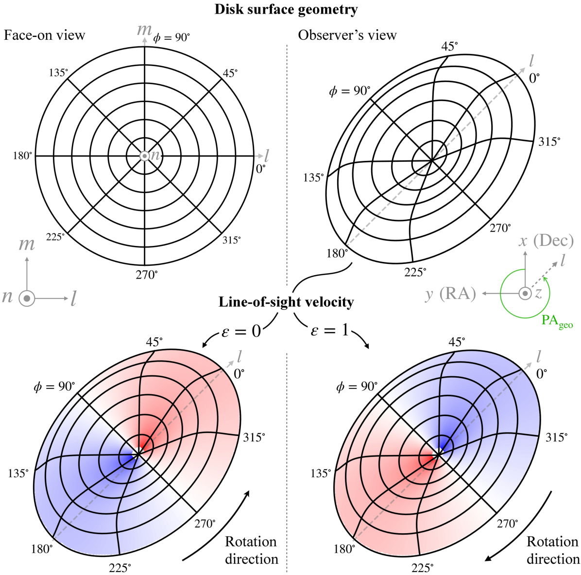
Figure 1. from Masataka Aizawa and Ryuta Orihara 2026 Astron. J. 171 doi:10.3847/1538-3881/ae1a75 https://dx.doi.org/10.3847/1538-3881/ae1a75 © 2025. The Author(s). Published by the American Astronomical Society.
