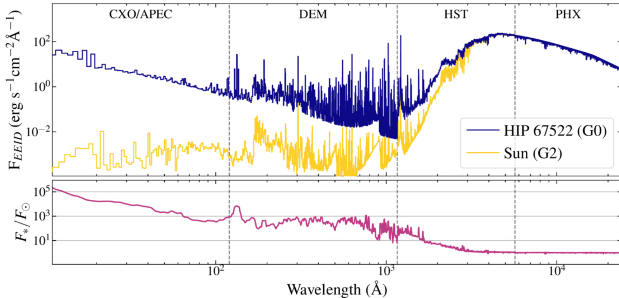
Figure 9. from Cynthia S. Froning et al 2026 Astron. J. 171 doi:10.3847/1538-3881/ae19ed https://dx.doi.org/10.3847/1538-3881/ae19ed © 2025. The Author(s). Published by the American Astronomical Society.
