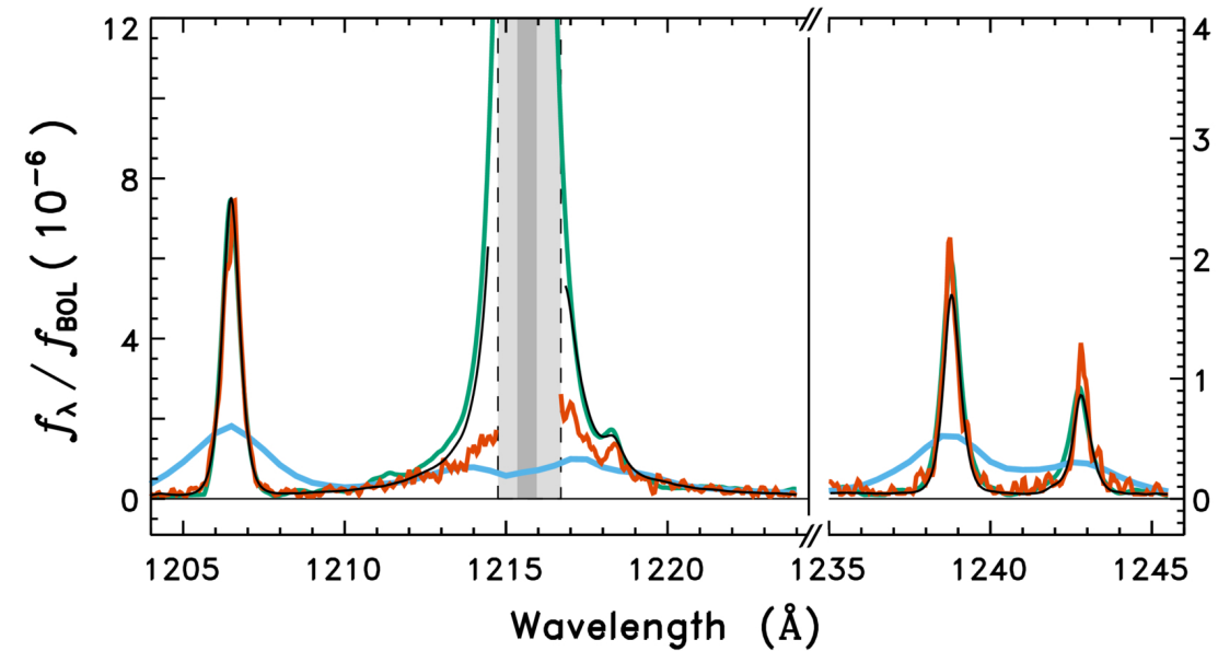
Figure 7. from Cynthia S. Froning et al 2026 Astron. J. 171 doi:10.3847/1538-3881/ae19ed https://dx.doi.org/10.3847/1538-3881/ae19ed © 2025. The Author(s). Published by the American Astronomical Society.
