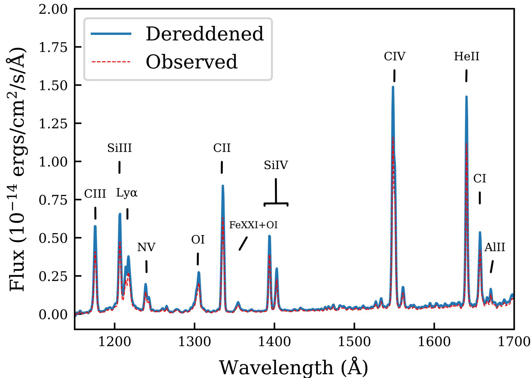
Figure 2. from Cynthia S. Froning et al 2026 Astron. J. 171 doi:10.3847/1538-3881/ae19ed https://dx.doi.org/10.3847/1538-3881/ae19ed © 2025. The Author(s). Published by the American Astronomical Society.
