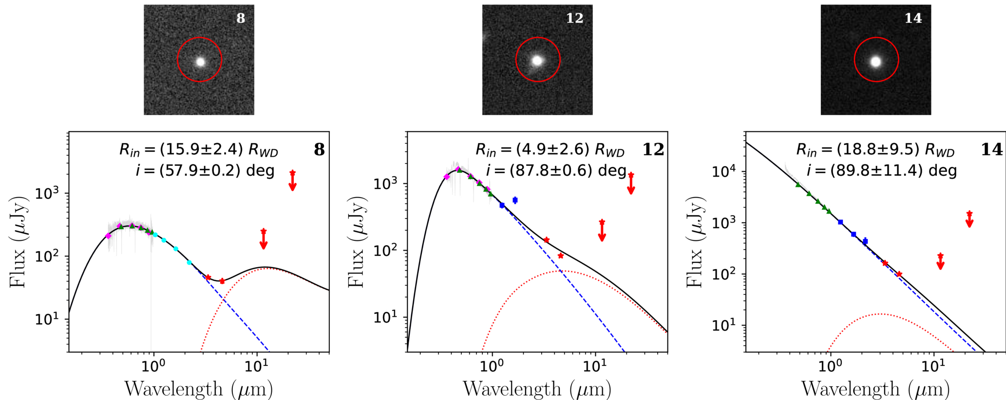
Figure 3. from Ziying Ma et al 2025 Astron. J. 170 doi:10.3847/1538-3881/ae197c https://dx.doi.org/10.3847/1538-3881/ae197c © 2025. The Author(s). Published by the American Astronomical Society.
