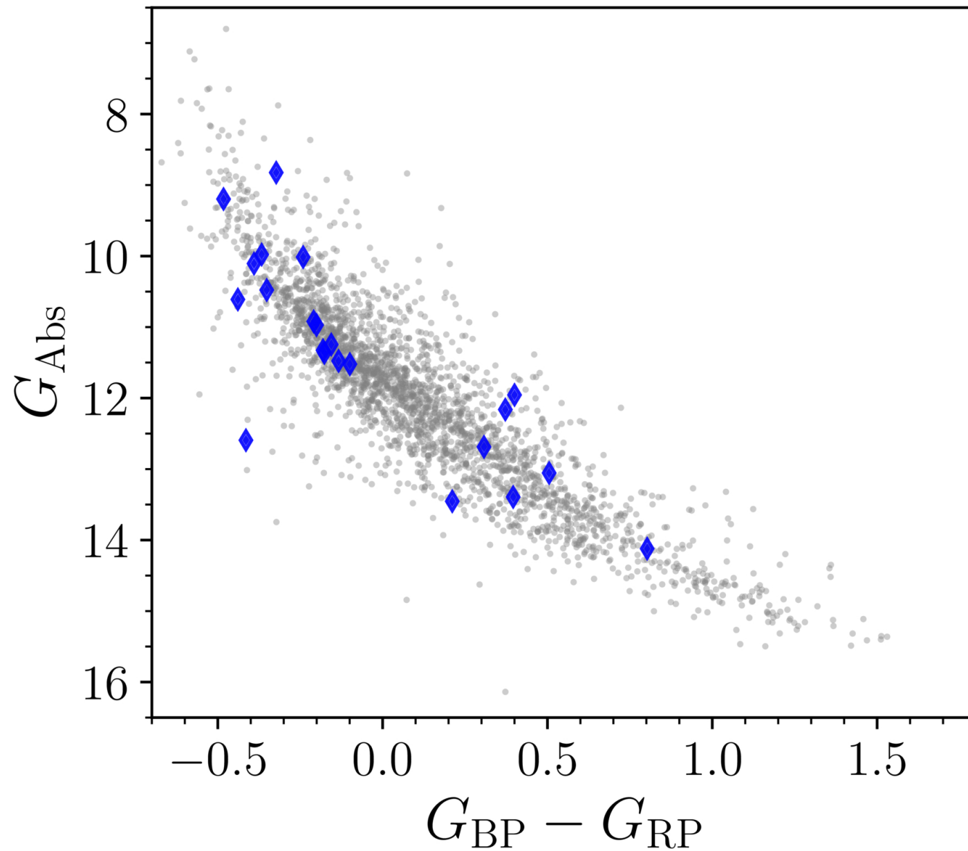
Figure 2. from Ziying Ma et al 2025 Astron. J. 170 doi:10.3847/1538-3881/ae197c https://dx.doi.org/10.3847/1538-3881/ae197c © 2025. The Author(s). Published by the American Astronomical Society.
