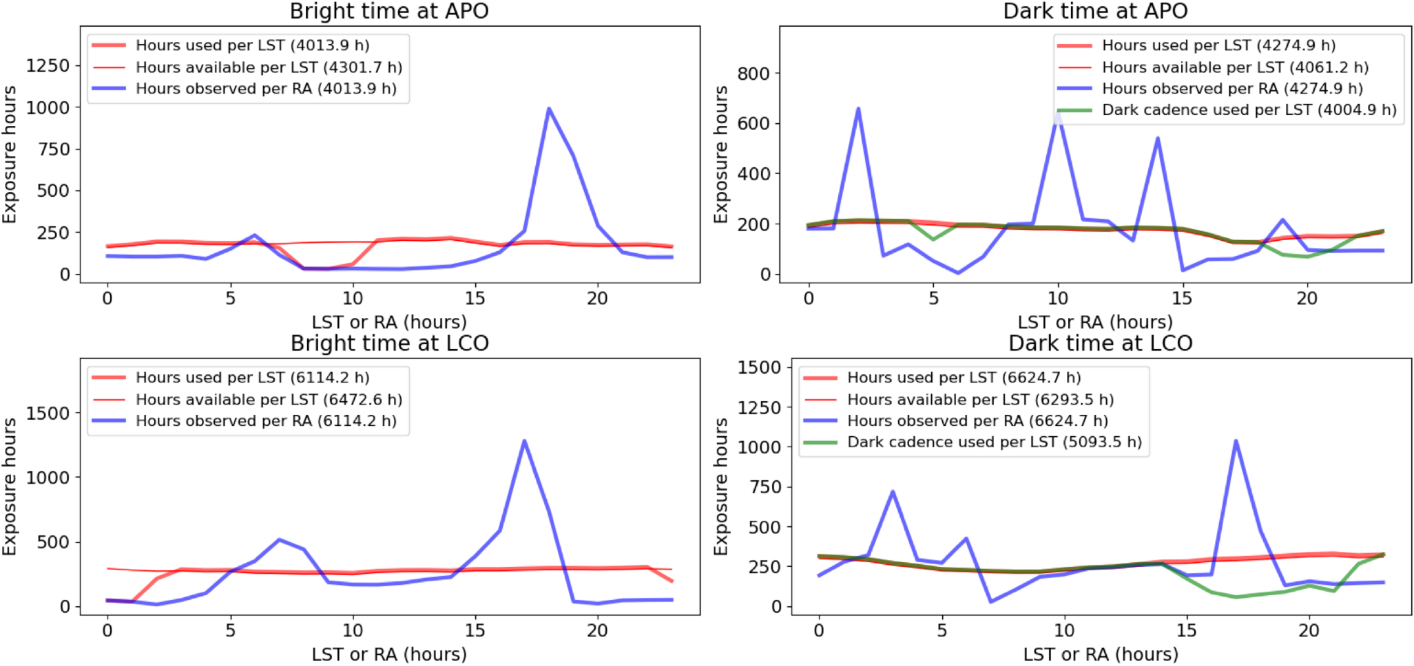
Figure 9. from Michael R. Blanton et al 2026 Astron. J. 171 doi:10.3847/1538-3881/ae196d https://dx.doi.org/10.3847/1538-3881/ae196d © 2025. The Author(s). Published by the American Astronomical Society.
