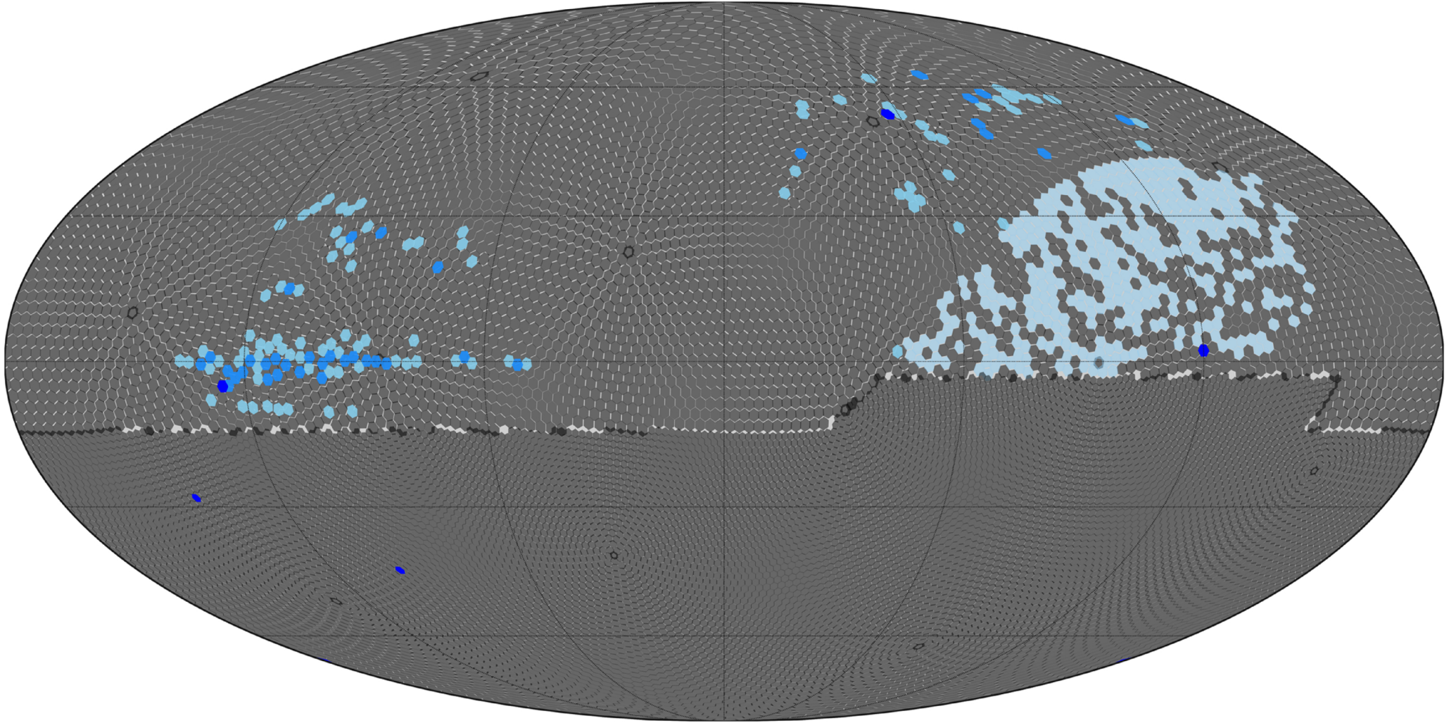
Figure 8. from Michael R. Blanton et al 2026 Astron. J. 171 doi:10.3847/1538-3881/ae196d https://dx.doi.org/10.3847/1538-3881/ae196d © 2025. The Author(s). Published by the American Astronomical Society.
