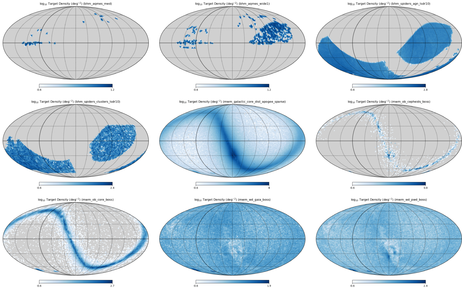
Figure 7. from Michael R. Blanton et al 2026 Astron. J. 171 doi:10.3847/1538-3881/ae196d https://dx.doi.org/10.3847/1538-3881/ae196d © 2025. The Author(s). Published by the American Astronomical Society.
