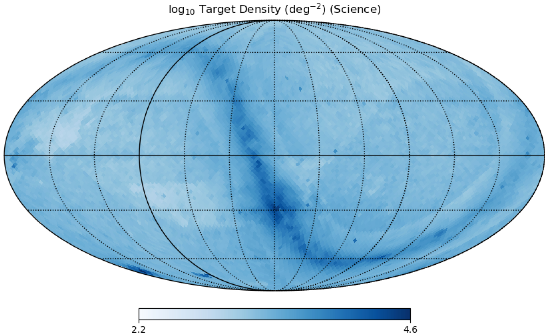
Figure 6. from Michael R. Blanton et al 2026 Astron. J. 171 doi:10.3847/1538-3881/ae196d https://dx.doi.org/10.3847/1538-3881/ae196d © 2025. The Author(s). Published by the American Astronomical Society.
