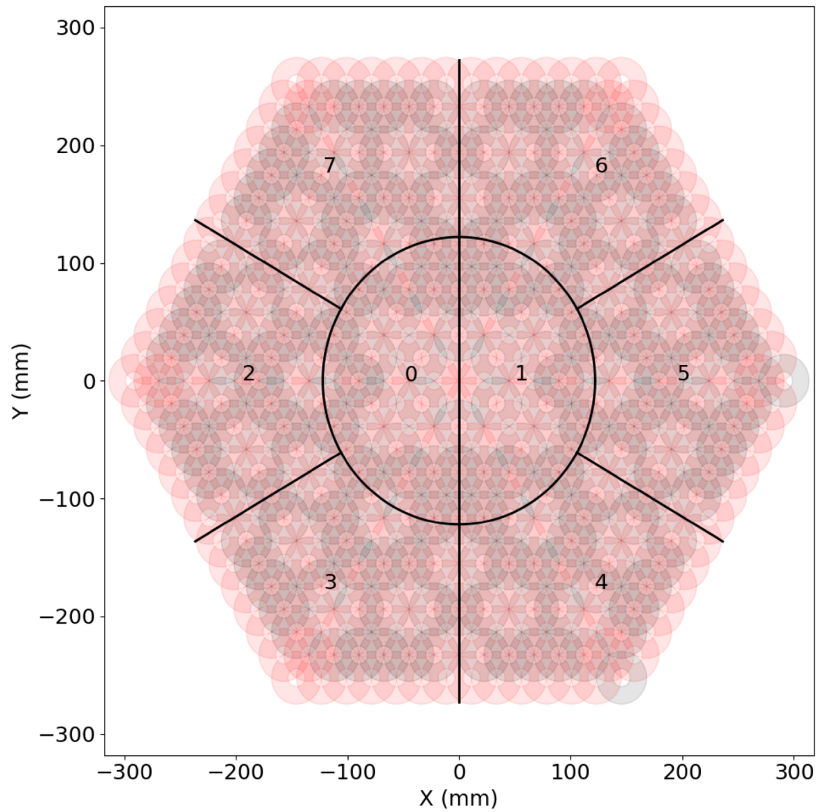
Figure 2. from Michael R. Blanton et al 2026 Astron. J. 171 doi:10.3847/1538-3881/ae196d https://dx.doi.org/10.3847/1538-3881/ae196d © 2025. The Author(s). Published by the American Astronomical Society.
