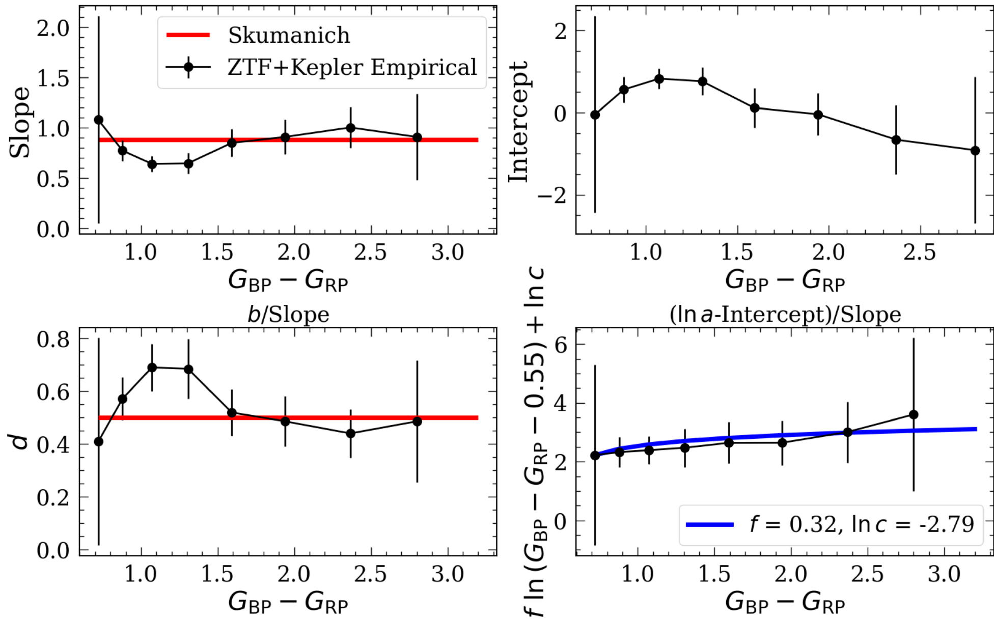
Figure 2. from Yuxi(Lucy) Lu et al 2026 Astron. J. 171 doi:10.3847/1538-3881/ae196b https://dx.doi.org/10.3847/1538-3881/ae196b © 2025. The Author(s). Published by the American Astronomical Society.
