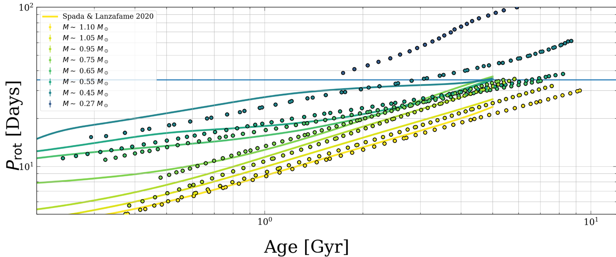
Figure 12. from Yuxi(Lucy) Lu et al 2026 Astron. J. 171 doi:10.3847/1538-3881/ae196b https://dx.doi.org/10.3847/1538-3881/ae196b © 2025. The Author(s). Published by the American Astronomical Society.
