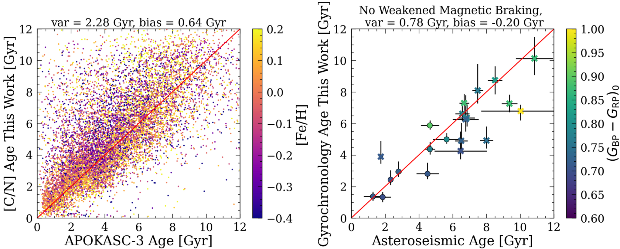
Figure 10. from Yuxi(Lucy) Lu et al 2026 Astron. J. 171 doi:10.3847/1538-3881/ae196b https://dx.doi.org/10.3847/1538-3881/ae196b © 2025. The Author(s). Published by the American Astronomical Society.
