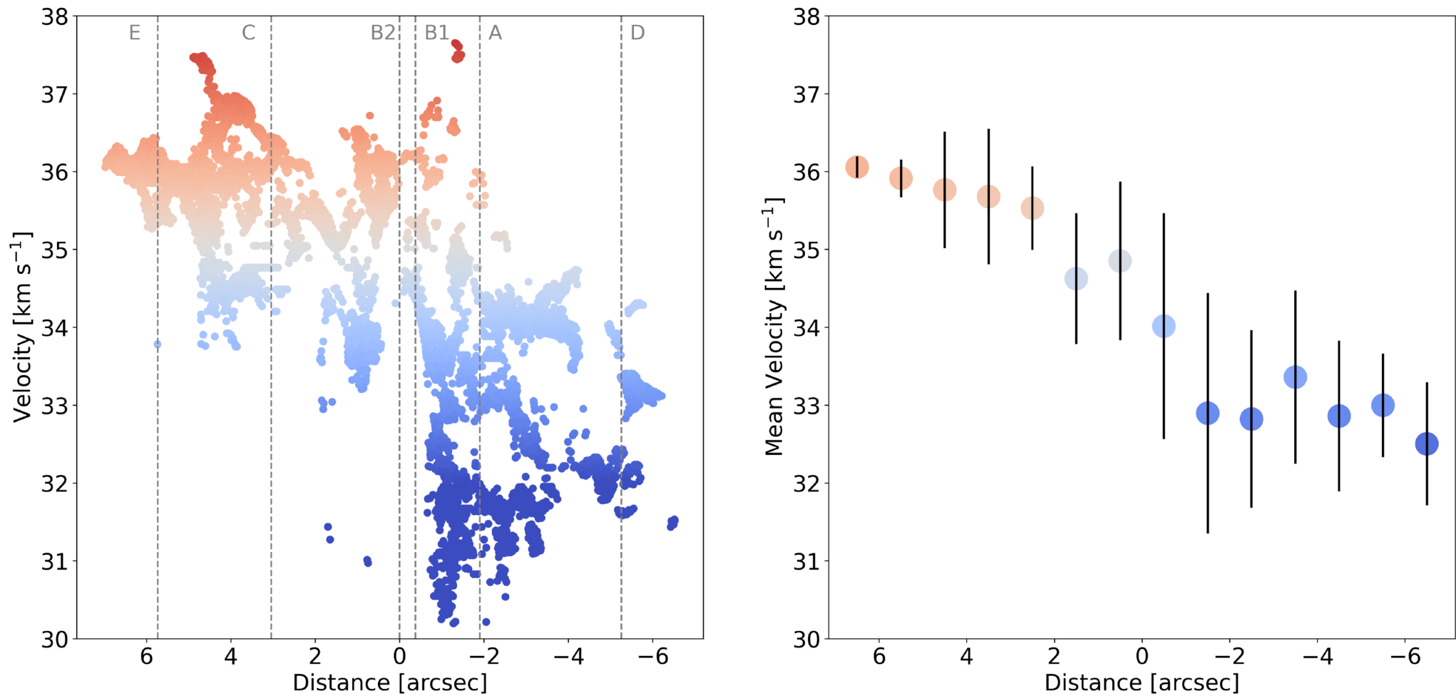
Figure 8. from Jihye Hwang et al 2026 Astron. J. 171 doi:10.3847/1538-3881/ae18c9 https://dx.doi.org/10.3847/1538-3881/ae18c9 © 2025. The Author(s). Published by the American Astronomical Society.
