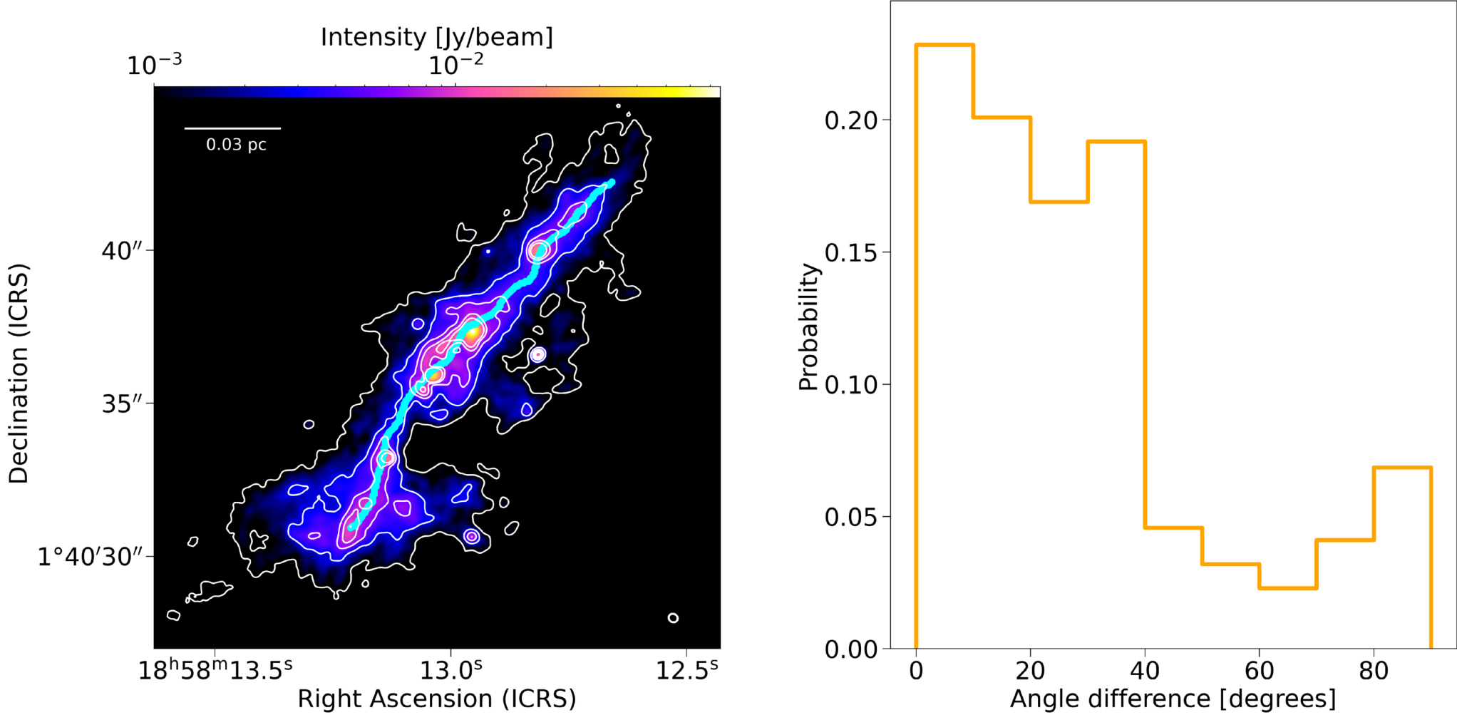
Figure 2. from Jihye Hwang et al 2026 Astron. J. 171 doi:10.3847/1538-3881/ae18c9 https://dx.doi.org/10.3847/1538-3881/ae18c9 © 2025. The Author(s). Published by the American Astronomical Society.
