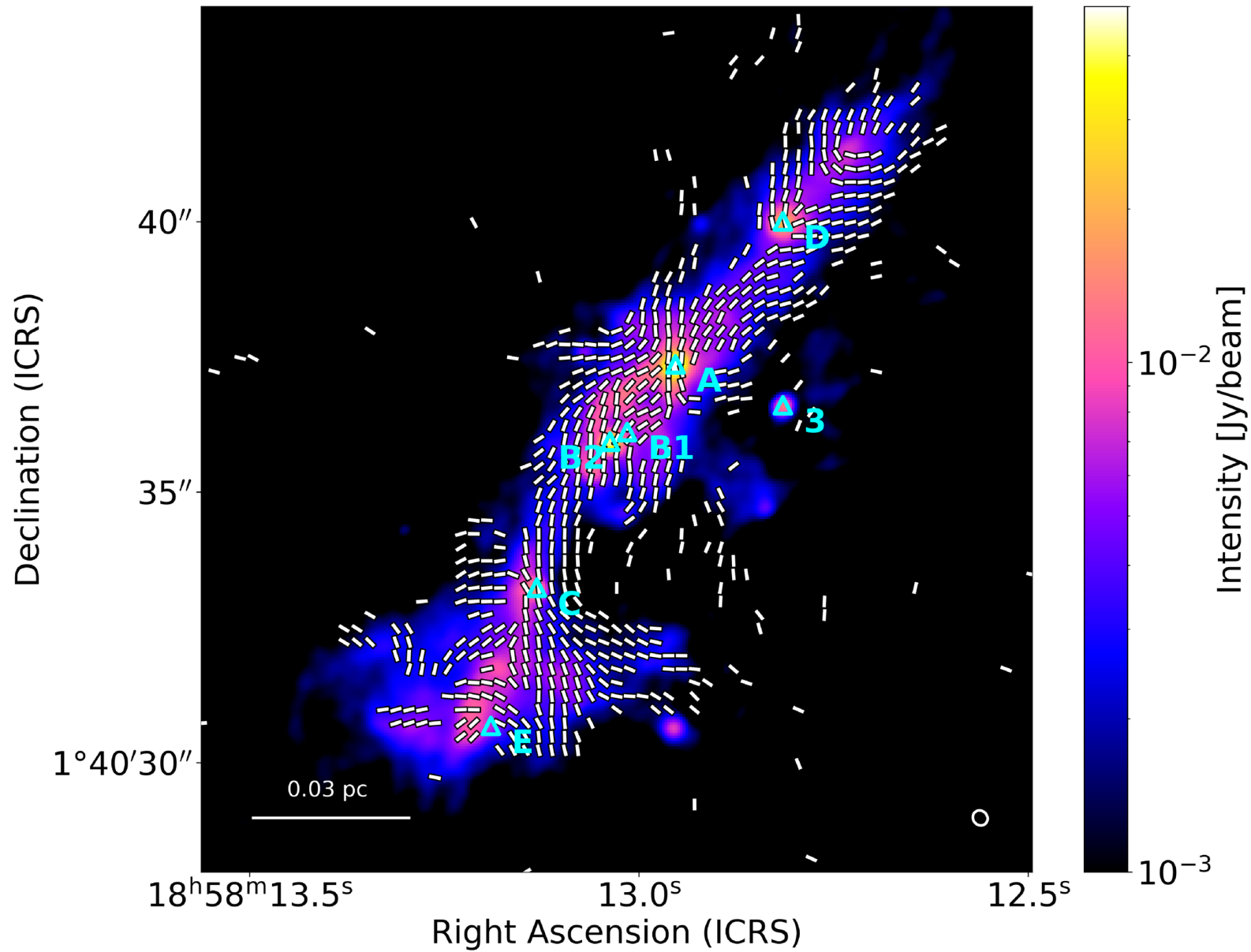
Figure 1. from Jihye Hwang et al 2026 Astron. J. 171 doi:10.3847/1538-3881/ae18c9 https://dx.doi.org/10.3847/1538-3881/ae18c9 © 2025. The Author(s). Published by the American Astronomical Society.
