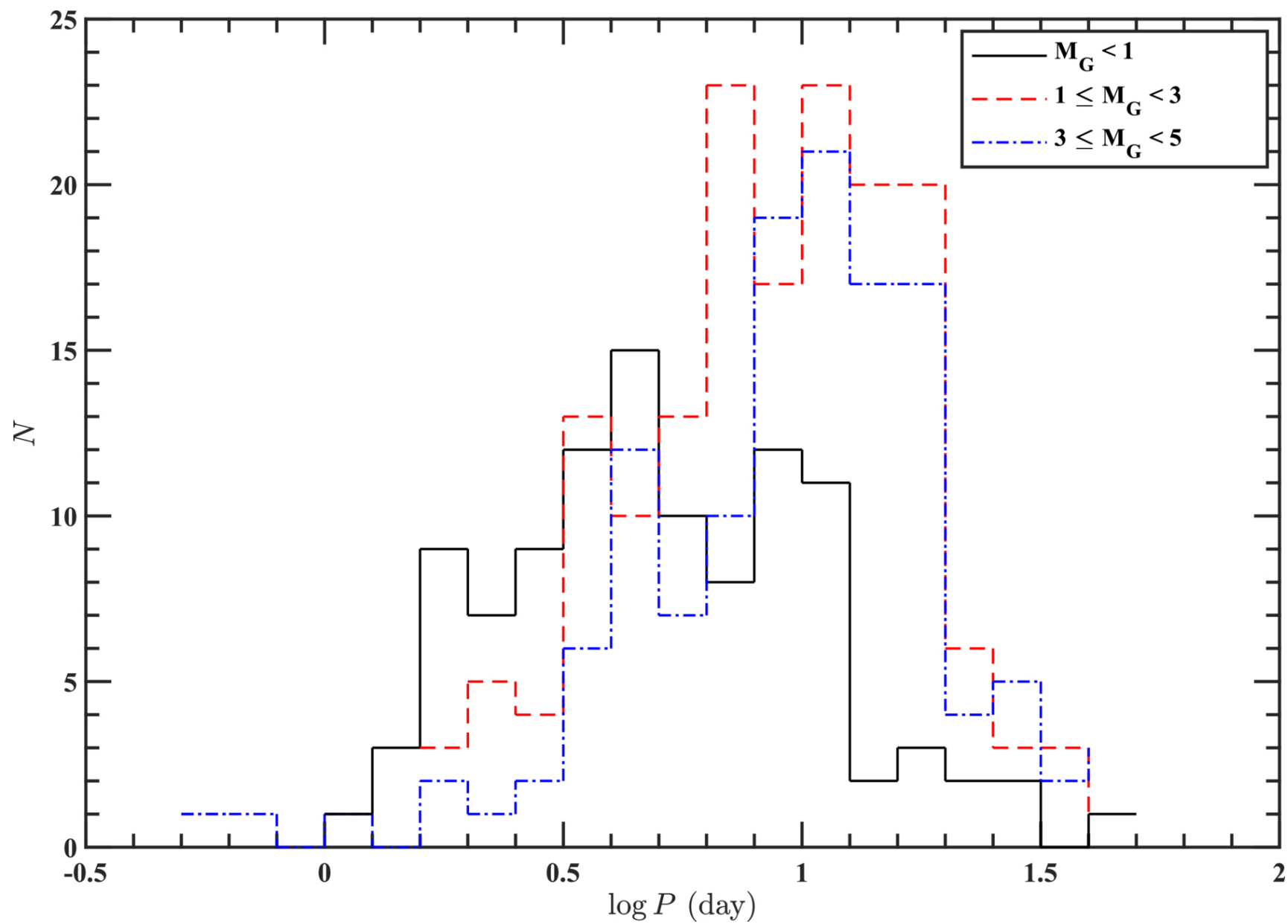
Figure 9. from Yanke Tang et al 2025 Astron. J. 170 doi:10.3847/1538-3881/ae18c4 https://dx.doi.org/10.3847/1538-3881/ae18c4 © 2025. The Author(s). Published by the American Astronomical Society.
