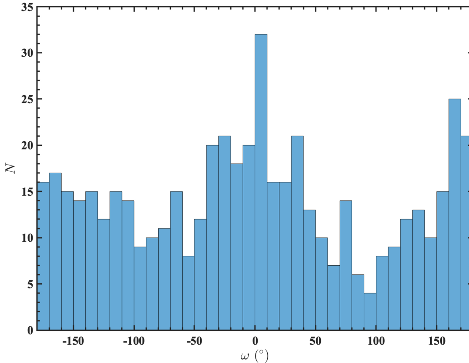
Figure 2. from Yanke Tang et al 2025 Astron. J. 170 doi:10.3847/1538-3881/ae18c4 https://dx.doi.org/10.3847/1538-3881/ae18c4 © 2025. The Author(s). Published by the American Astronomical Society.
