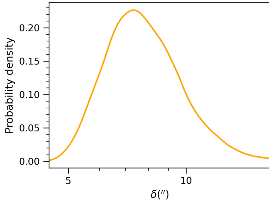
Figure 3. from Yiyang Guo et al 2025 Astron. J. 170 doi:10.3847/1538-3881/ae1833 https://dx.doi.org/10.3847/1538-3881/ae1833 © 2025. The Author(s). Published by the American Astronomical Society.
