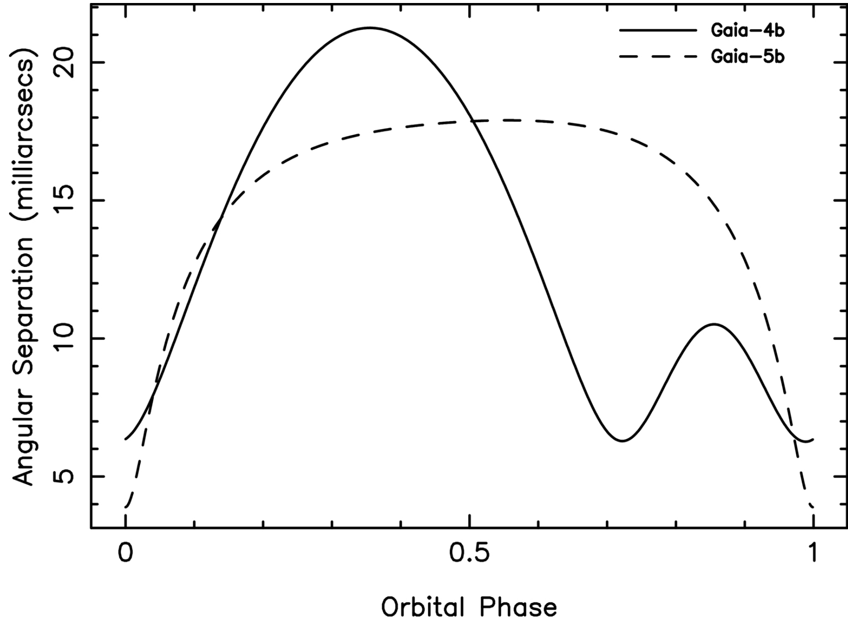
Figure 5. from Stephen R. Kane 2025 Astron. J. 170 doi:10.3847/1538-3881/ae17c9 https://dx.doi.org/10.3847/1538-3881/ae17c9 © 2025. The Author(s). Published by the American Astronomical Society.
