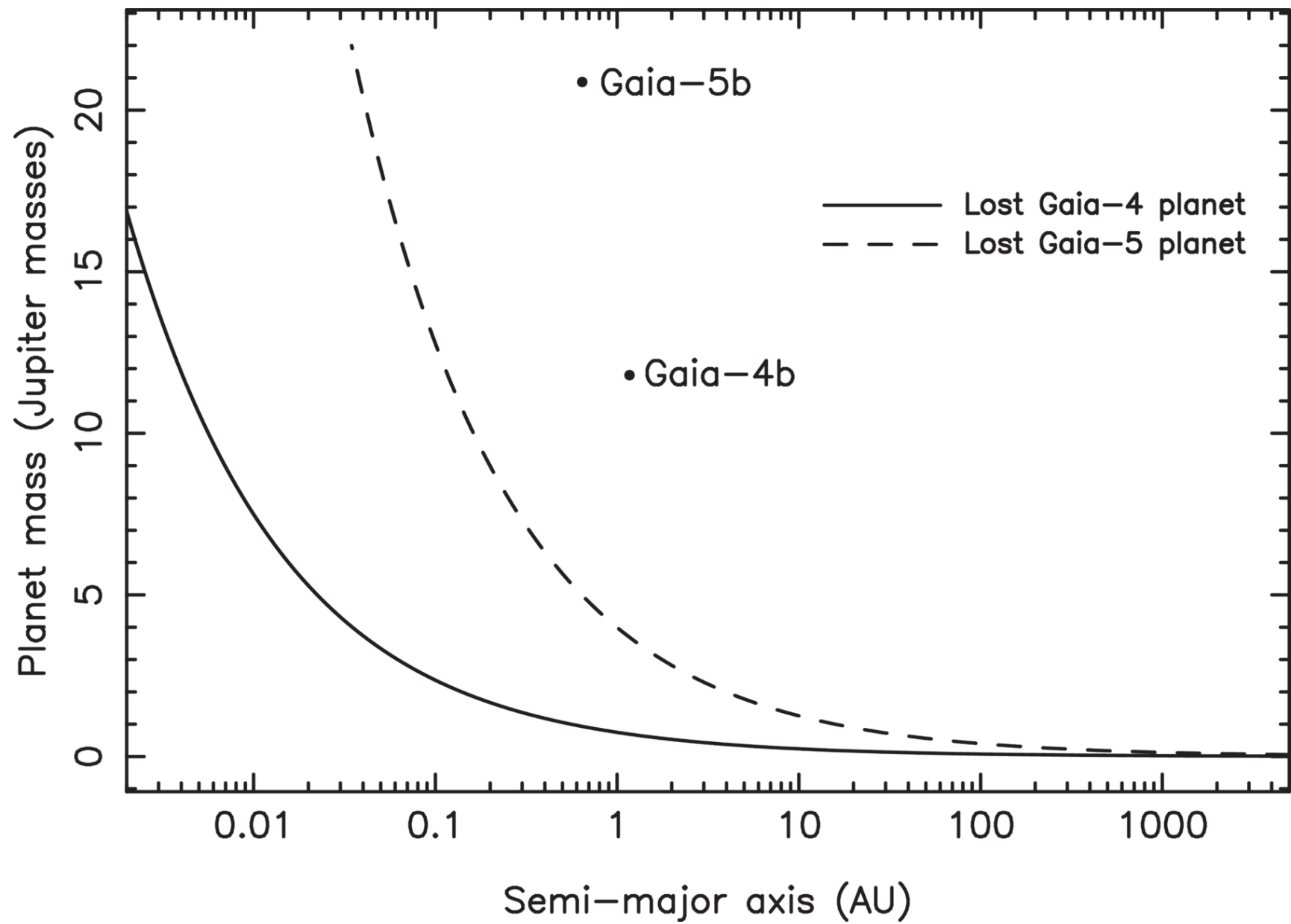
Figure 3. from Stephen R. Kane 2025 Astron. J. 170 doi:10.3847/1538-3881/ae17c9 https://dx.doi.org/10.3847/1538-3881/ae17c9 © 2025. The Author(s). Published by the American Astronomical Society.
