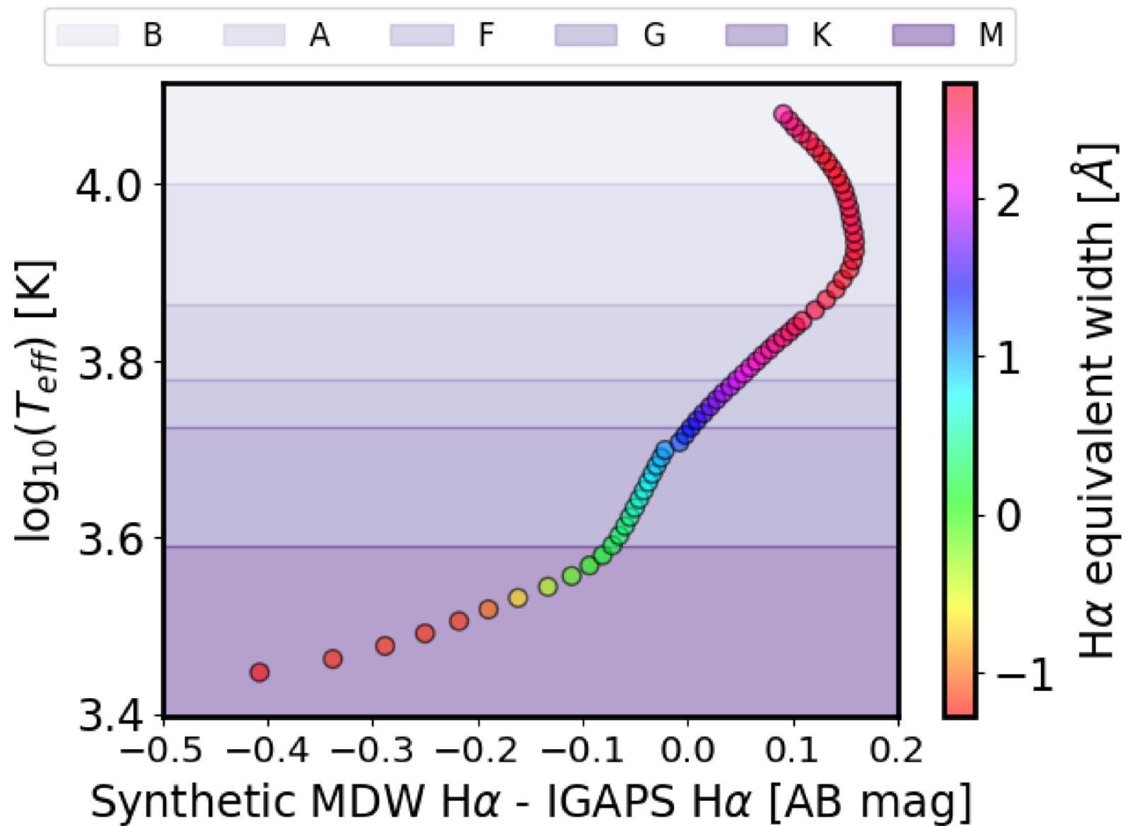
Figure 6. from Noor Aftab et al 2026 Astron. J. 171 doi:10.3847/1538-3881/ae17b4 https://dx.doi.org/10.3847/1538-3881/ae17b4 © 2025. The Author(s). Published by the American Astronomical Society.
