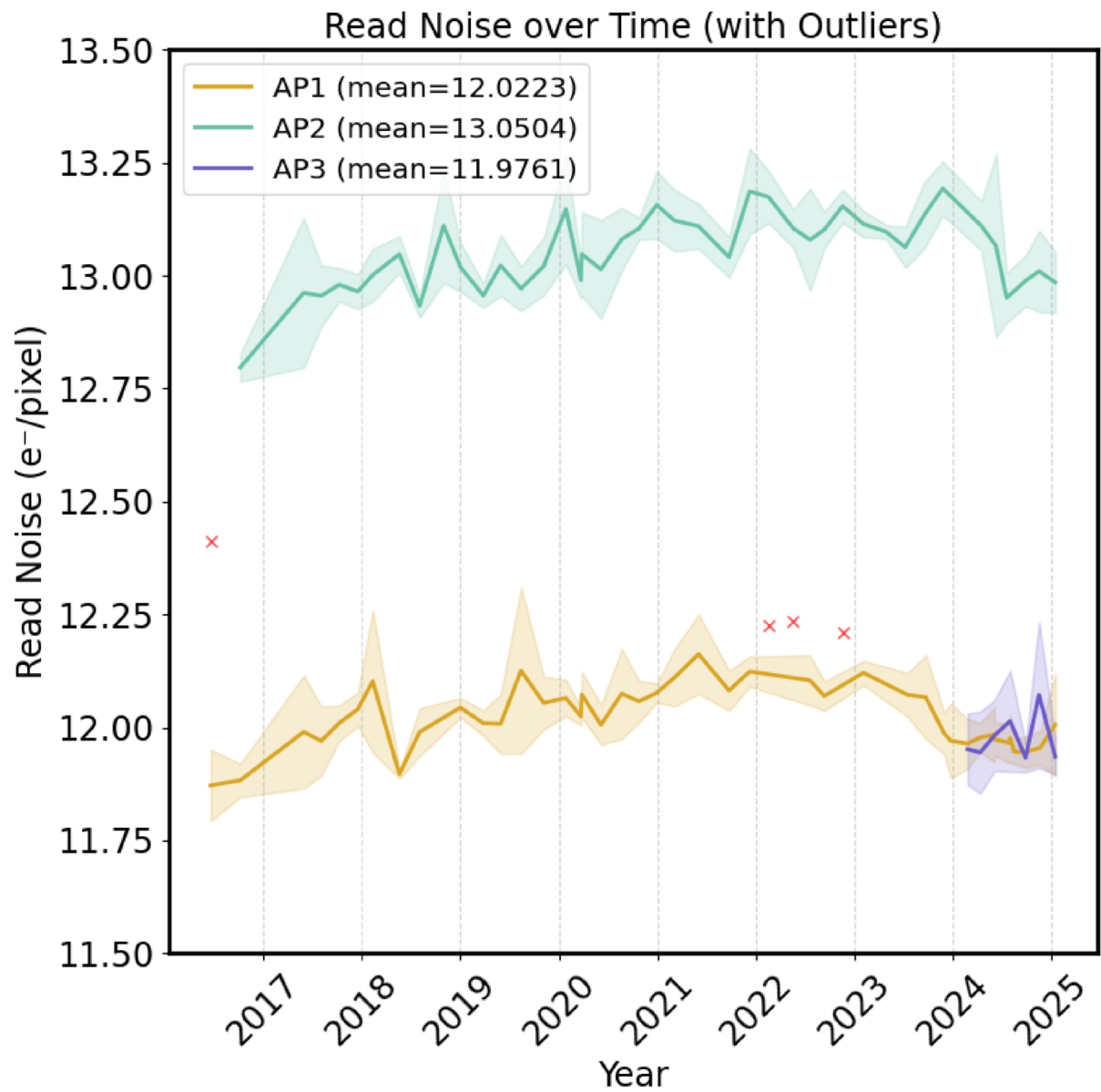
Figure 22. from Noor Aftab et al 2026 Astron. J. 171 doi:10.3847/1538-3881/ae17b4 https://dx.doi.org/10.3847/1538-3881/ae17b4 © 2025. The Author(s). Published by the American Astronomical Society.
