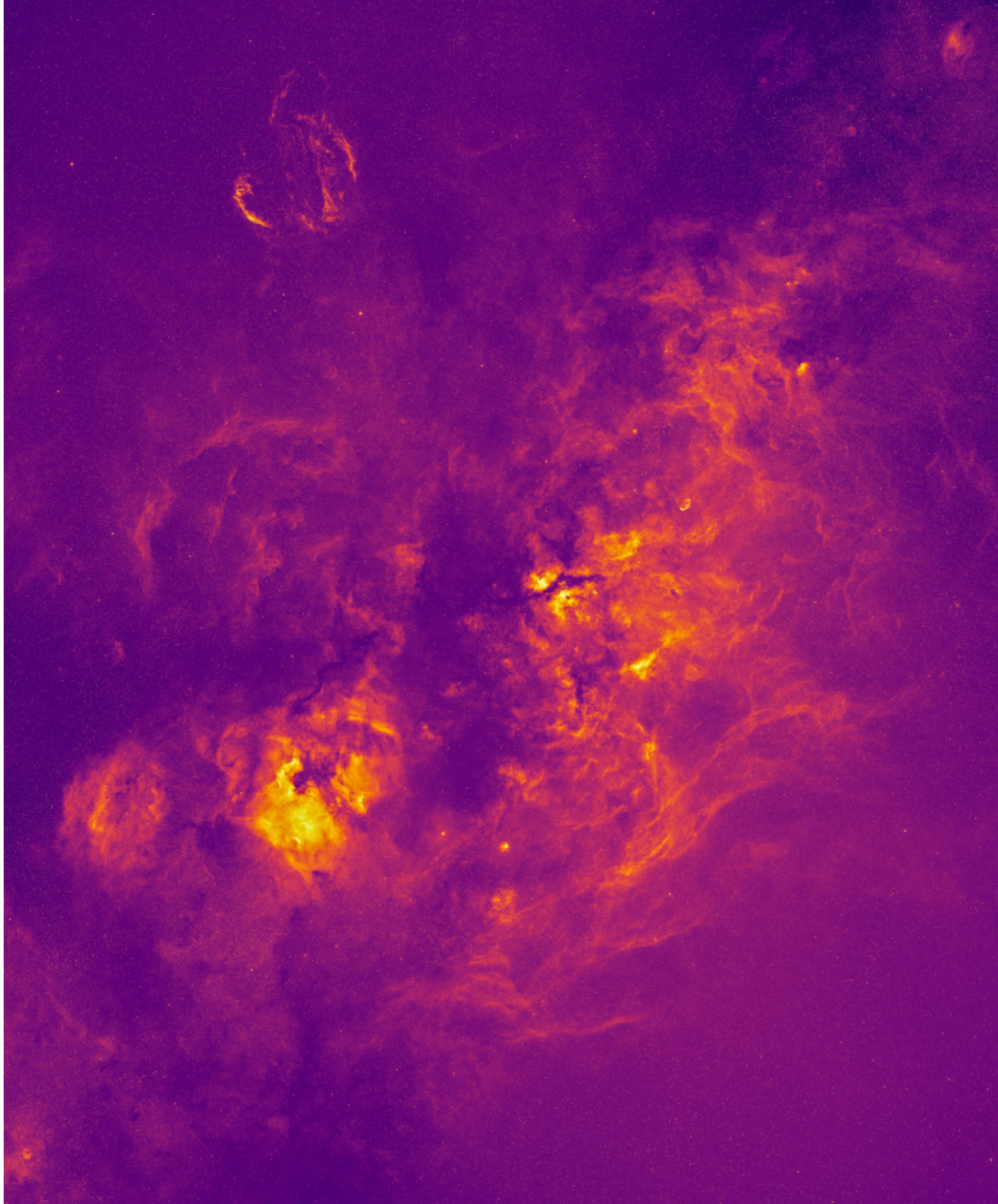
Figure 20. from Noor Aftab et al 2026 Astron. J. 171 doi:10.3847/1538-3881/ae17b4 https://dx.doi.org/10.3847/1538-3881/ae17b4 © 2025. The Author(s). Published by the American Astronomical Society.
