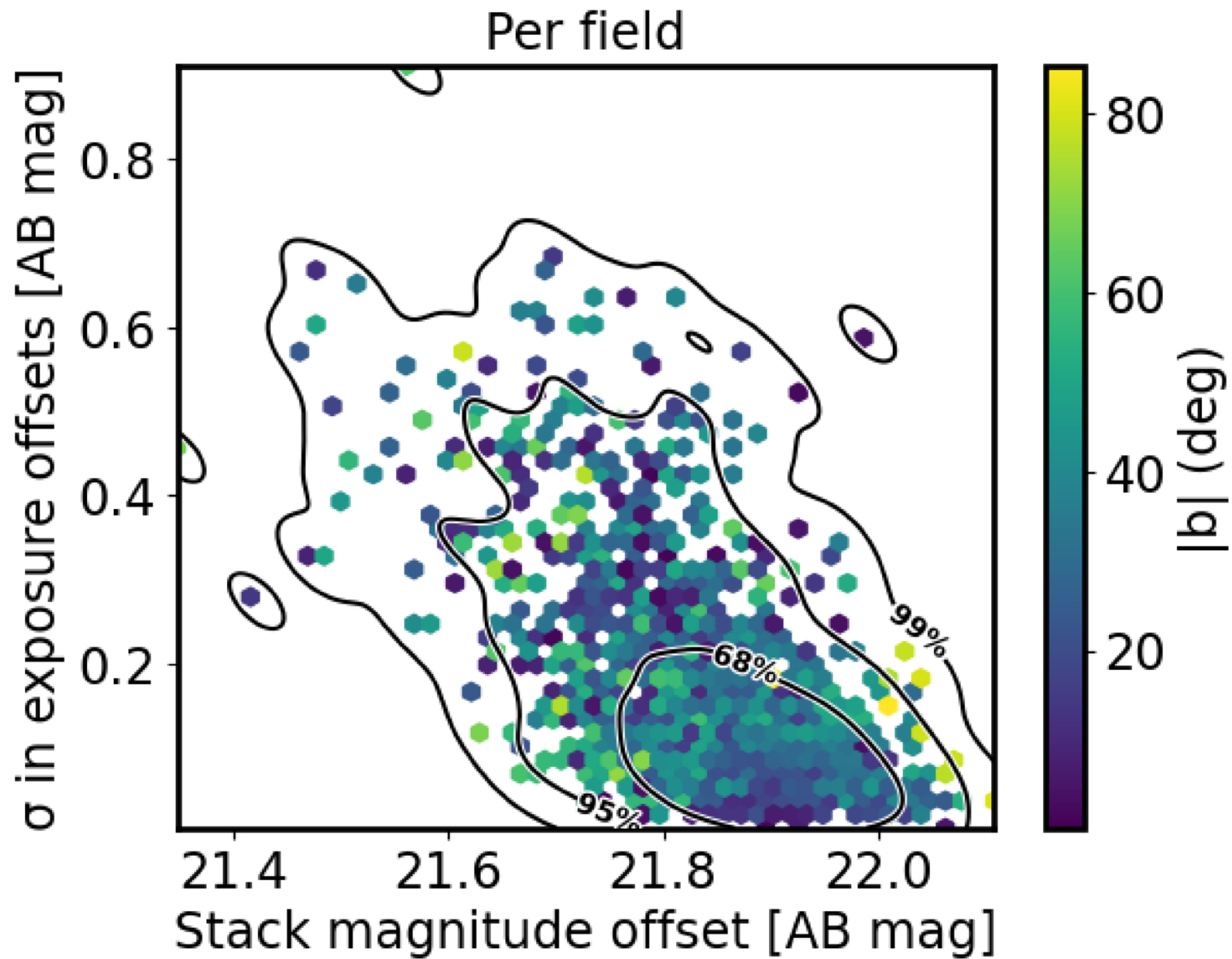
Figure 19. from Noor Aftab et al 2026 Astron. J. 171 doi:10.3847/1538-3881/ae17b4 https://dx.doi.org/10.3847/1538-3881/ae17b4 © 2025. The Author(s). Published by the American Astronomical Society.
