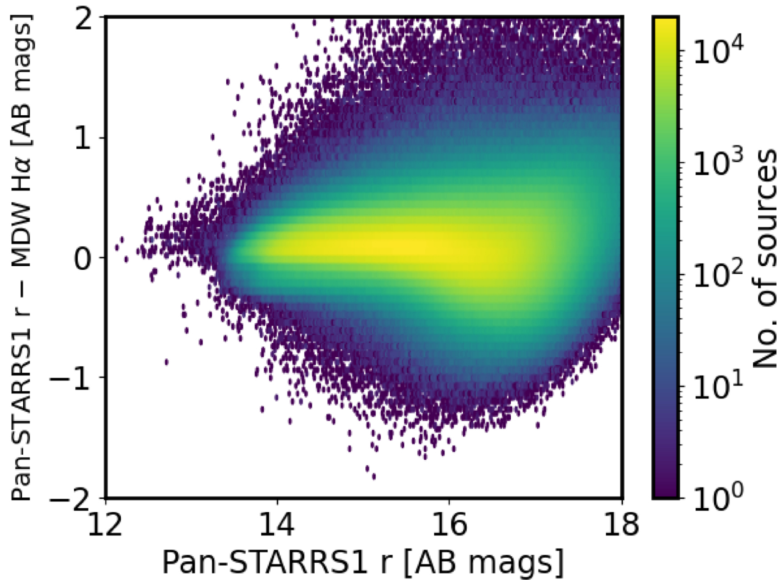
Figure 18. from Noor Aftab et al 2026 Astron. J. 171 doi:10.3847/1538-3881/ae17b4 https://dx.doi.org/10.3847/1538-3881/ae17b4 © 2025. The Author(s). Published by the American Astronomical Society.
