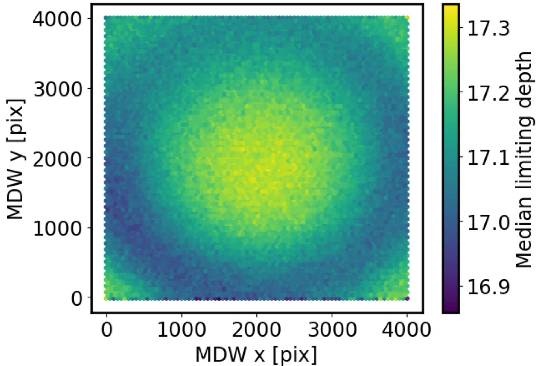
Figure 15. from Noor Aftab et al 2026 Astron. J. 171 doi:10.3847/1538-3881/ae17b4 https://dx.doi.org/10.3847/1538-3881/ae17b4 © 2025. The Author(s). Published by the American Astronomical Society.
