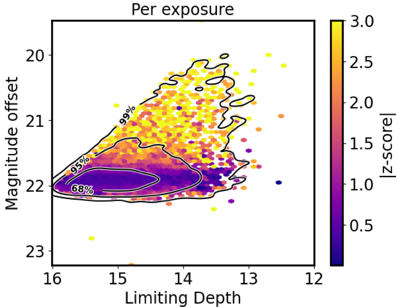
Figure 13. from Noor Aftab et al 2026 Astron. J. 171 doi:10.3847/1538-3881/ae17b4 https://dx.doi.org/10.3847/1538-3881/ae17b4 © 2025. The Author(s). Published by the American Astronomical Society.
