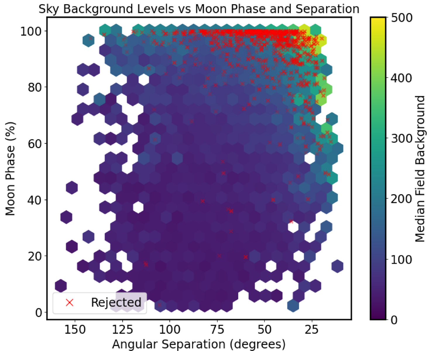
Figure 12. from Noor Aftab et al 2026 Astron. J. 171 doi:10.3847/1538-3881/ae17b4 https://dx.doi.org/10.3847/1538-3881/ae17b4 © 2025. The Author(s). Published by the American Astronomical Society.
