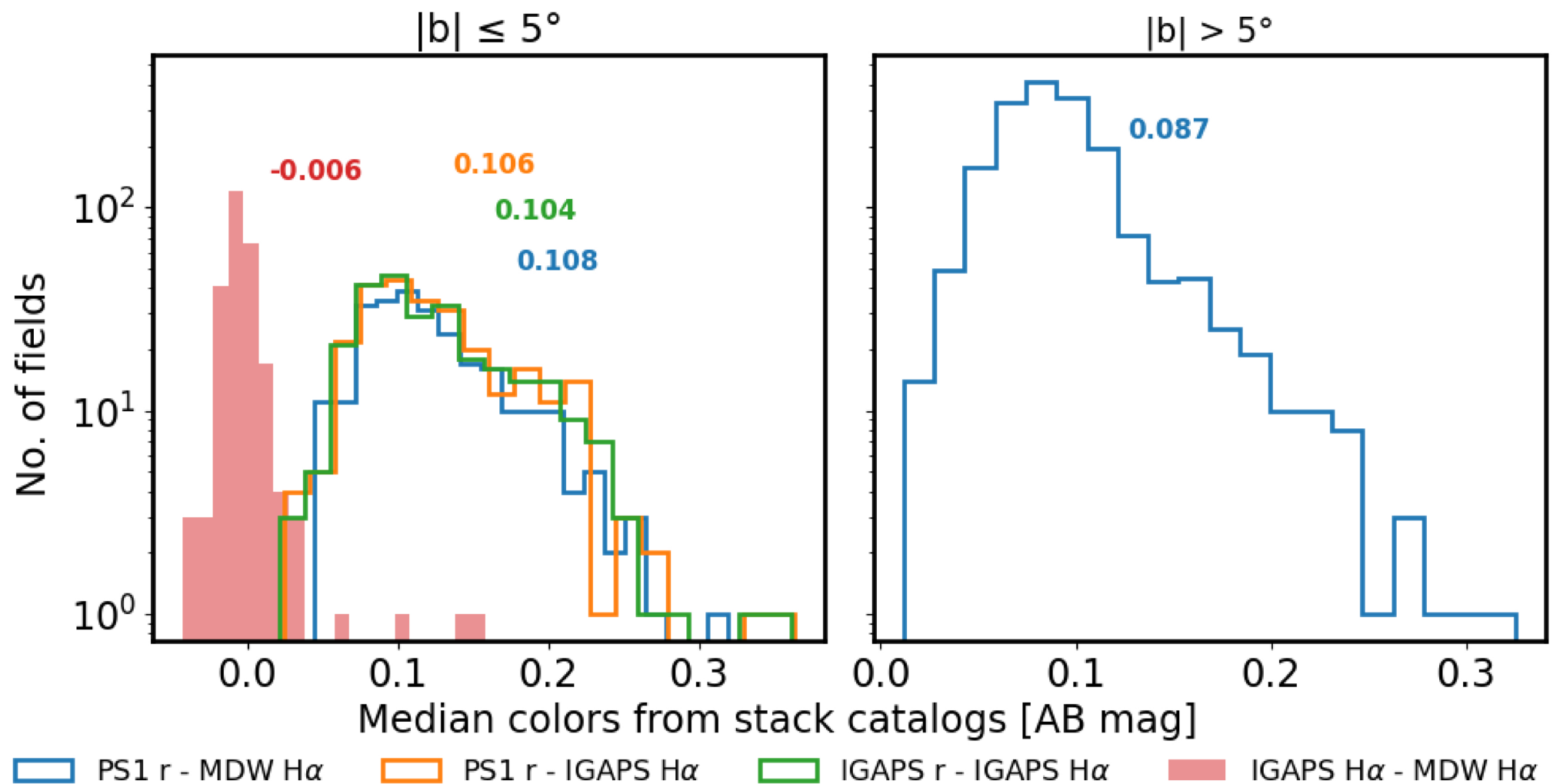
Figure 11. from Noor Aftab et al 2026 Astron. J. 171 doi:10.3847/1538-3881/ae17b4 https://dx.doi.org/10.3847/1538-3881/ae17b4 © 2025. The Author(s). Published by the American Astronomical Society.
