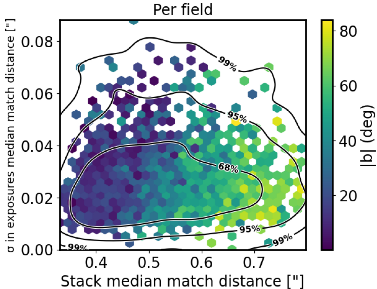
Figure 10. from Noor Aftab et al 2026 Astron. J. 171 doi:10.3847/1538-3881/ae17b4 https://dx.doi.org/10.3847/1538-3881/ae17b4 © 2025. The Author(s). Published by the American Astronomical Society.
