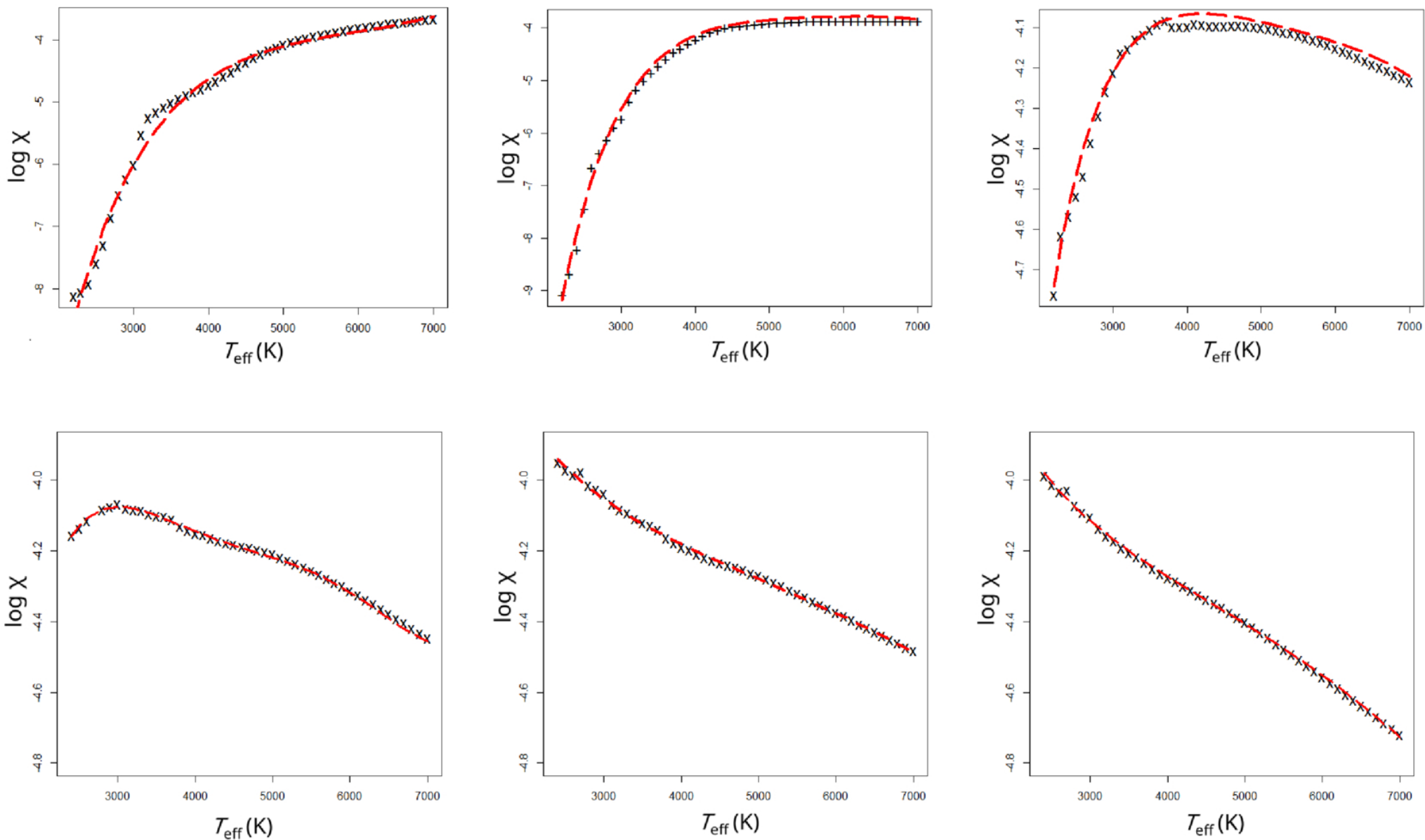
Figure 8. from Fernando Labarga and David Montes 2026 Astron. J. 171 doi:10.3847/1538-3881/ae173e https://dx.doi.org/10.3847/1538-3881/ae173e © 2025. The Author(s). Published by the American Astronomical Society.
