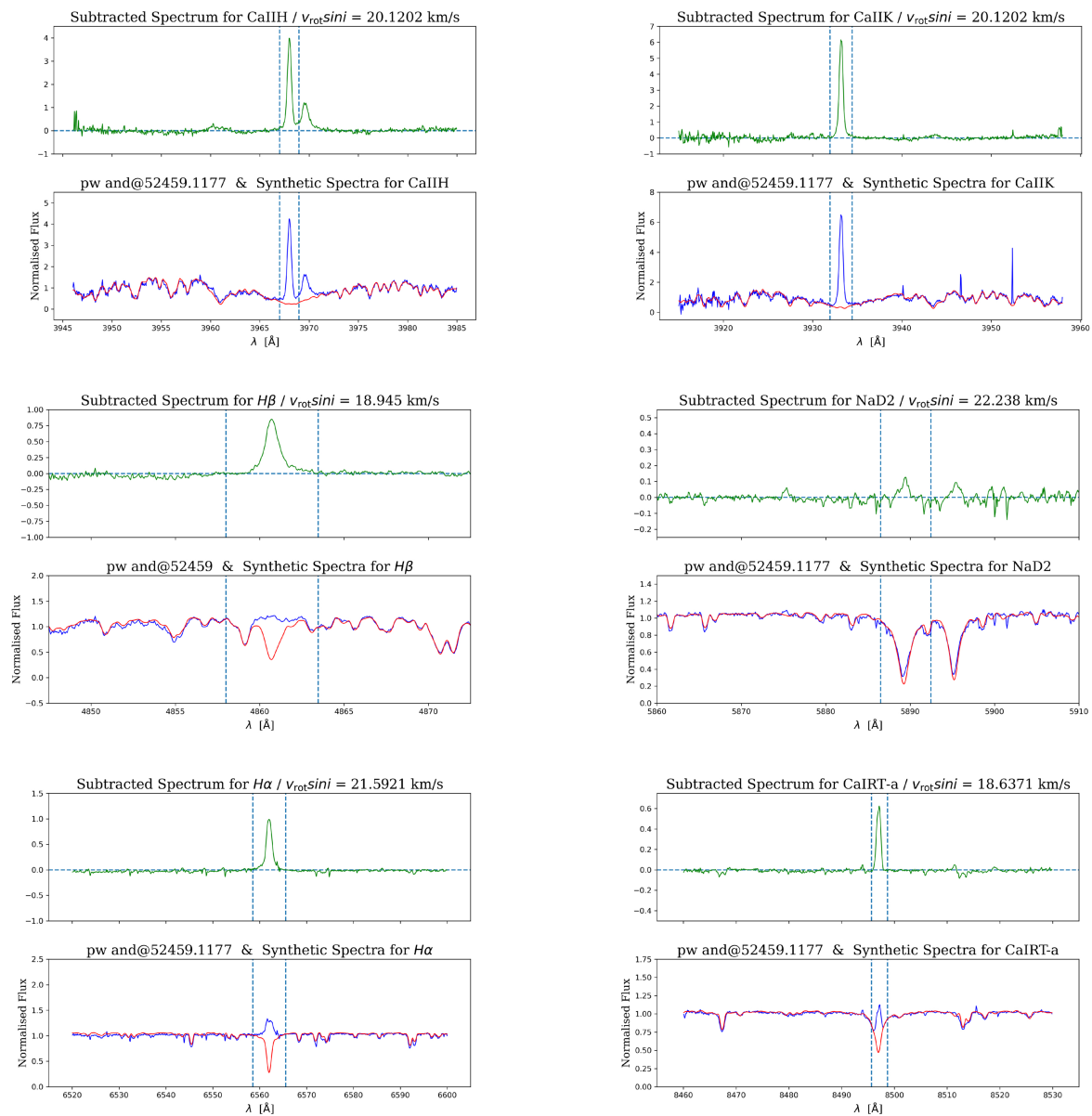
Figure 5. from Fernando Labarga and David Montes 2026 Astron. J. 171 doi:10.3847/1538-3881/ae173e https://dx.doi.org/10.3847/1538-3881/ae173e © 2025. The Author(s). Published by the American Astronomical Society.
