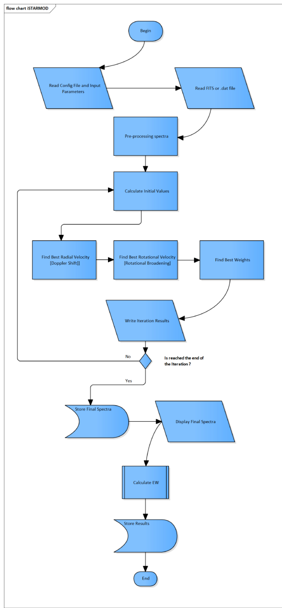
Figure 3. from Fernando Labarga and David Montes 2026 Astron. J. 171 doi:10.3847/1538-3881/ae173e https://dx.doi.org/10.3847/1538-3881/ae173e © 2025. The Author(s). Published by the American Astronomical Society.
