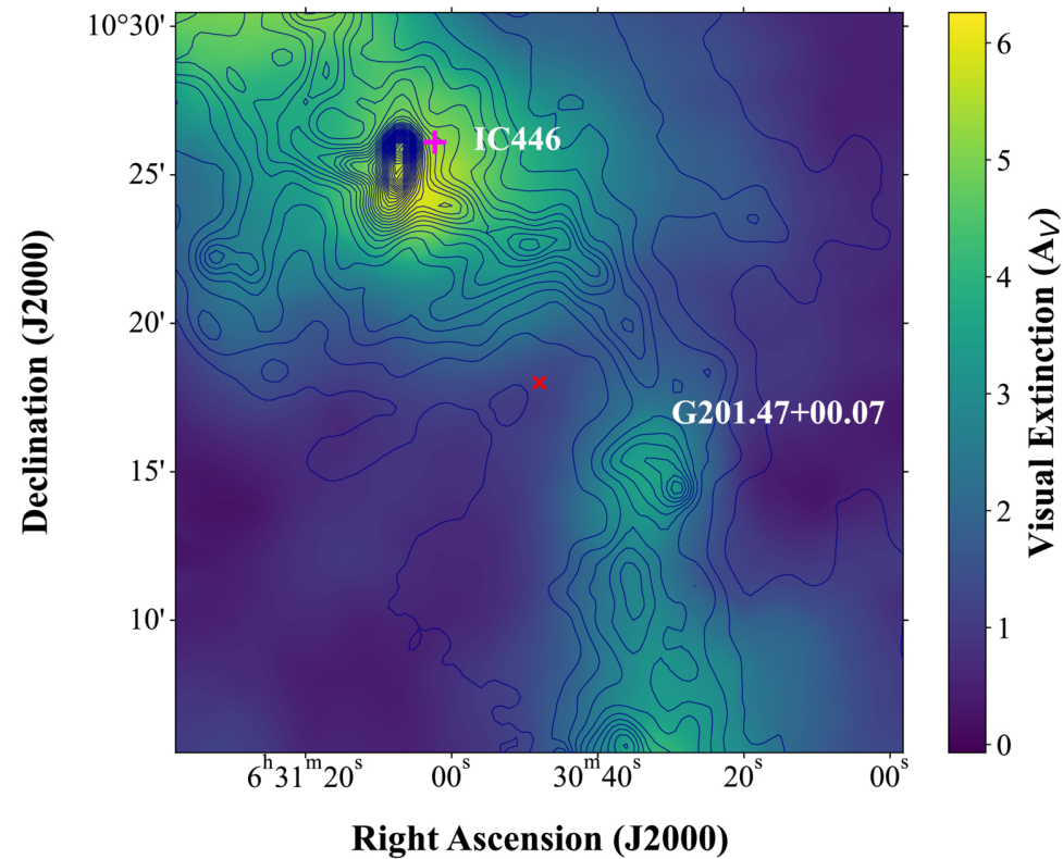
(b) Extinction map for L1607
