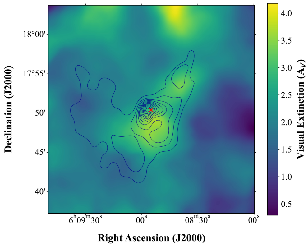
(a) Extinction map for L1578
