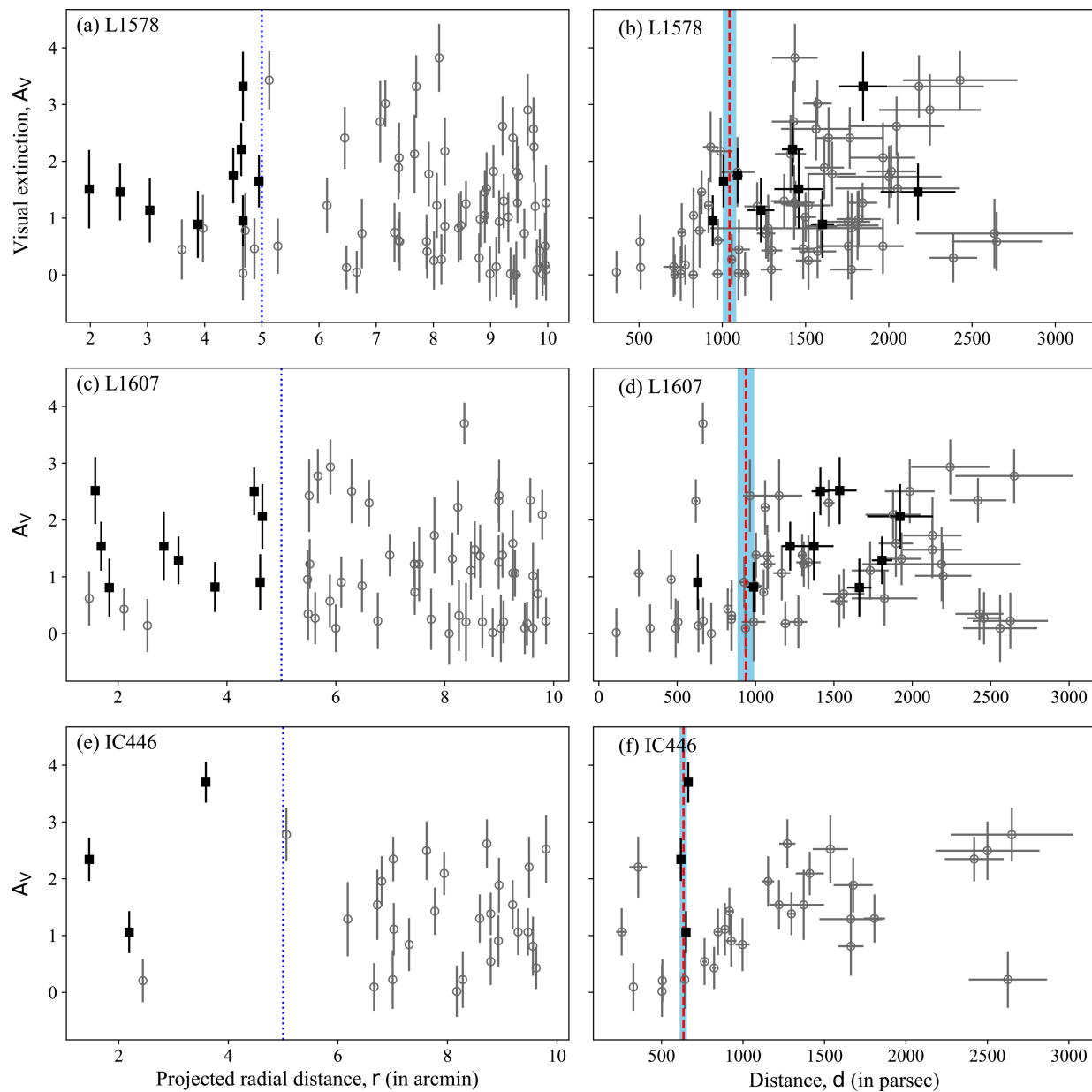
Figure 1. from Sanchali Nath Mazumdar et al 2026 Astron. J. 171 doi:10.3847/1538-3881/ae169c https://dx.doi.org/10.3847/1538-3881/ae169c © 2025. The Author(s). Published by the American Astronomical Society.
