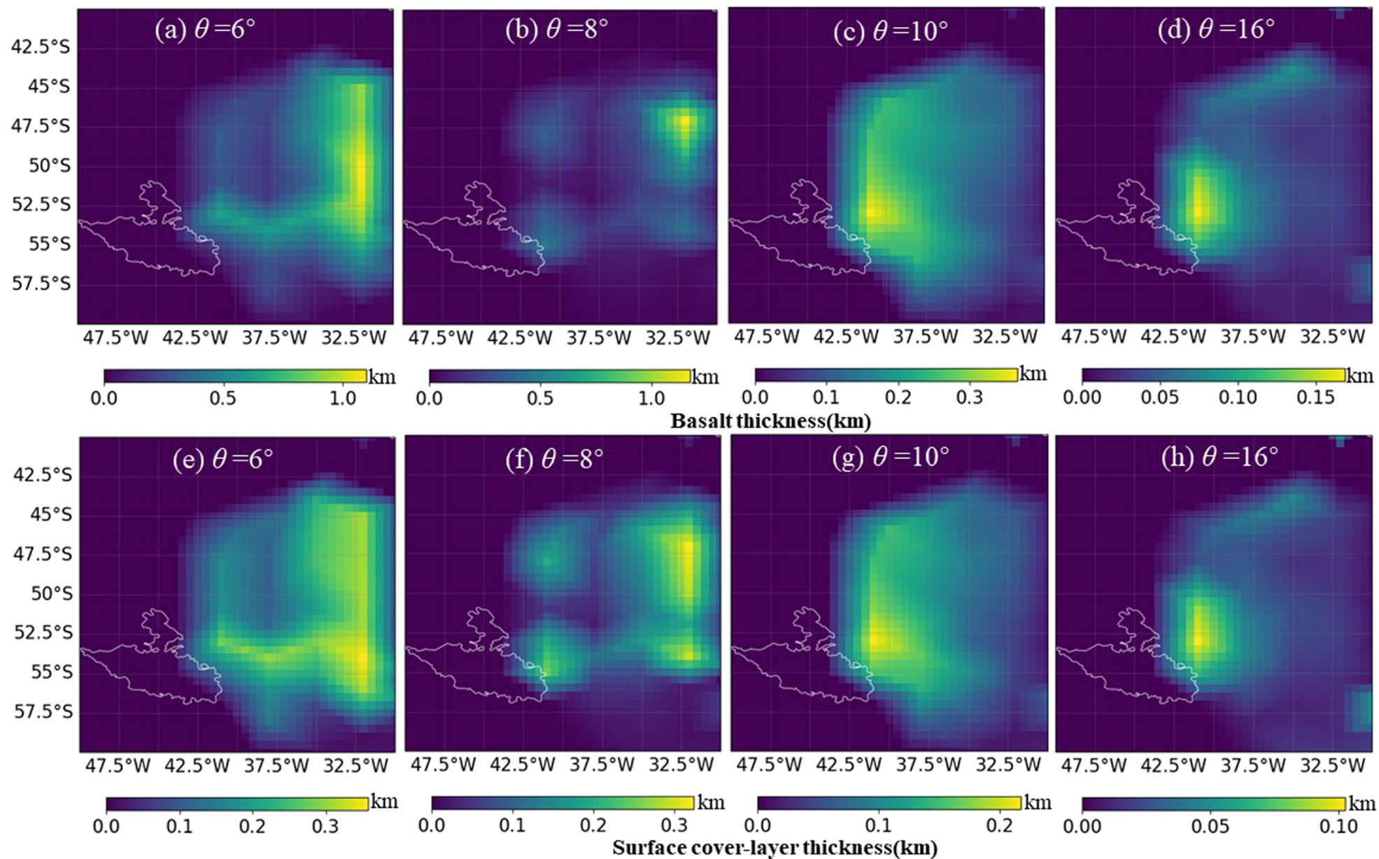
Figure 9. from Wensong Zhang et al 2026 Astron. J. 171 doi:10.3847/1538-3881/ae168d https://dx.doi.org/10.3847/1538-3881/ae168d © 2025. The Author(s). Published by the American Astronomical Society.
