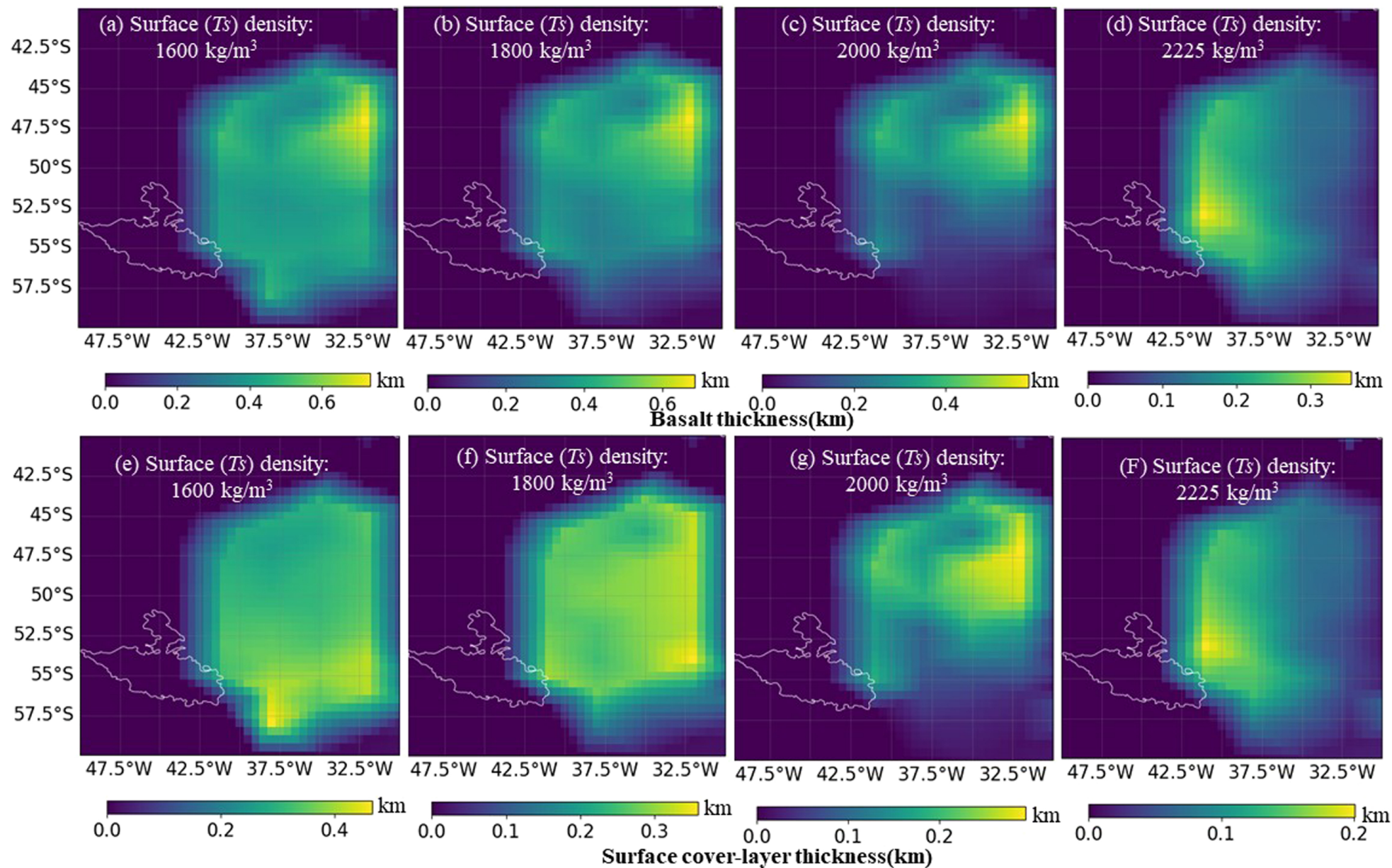
Figure 7. from Wensong Zhang et al 2026 Astron. J. 171 doi:10.3847/1538-3881/ae168d https://dx.doi.org/10.3847/1538-3881/ae168d © 2025. The Author(s). Published by the American Astronomical Society.
