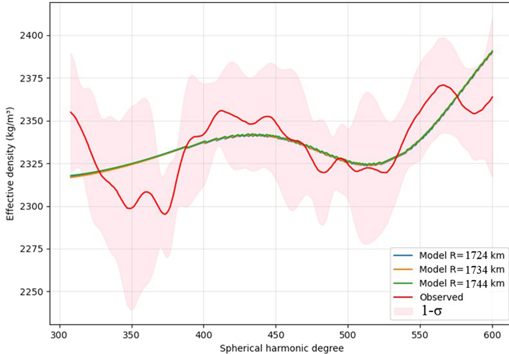
Figure 5. from Wensong Zhang et al 2026 Astron. J. 171 doi:10.3847/1538-3881/ae168d https://dx.doi.org/10.3847/1538-3881/ae168d © 2025. The Author(s). Published by the American Astronomical Society.
