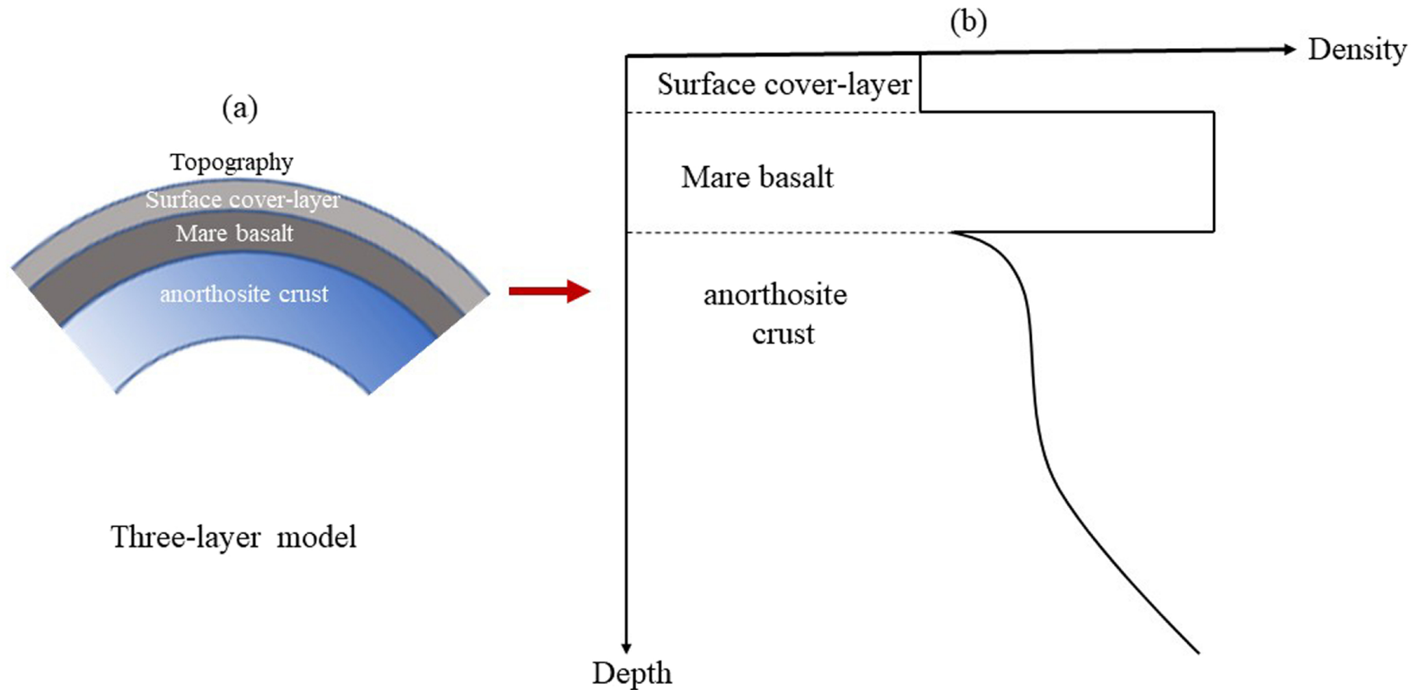
Figure 2. from Wensong Zhang et al 2026 Astron. J. 171 doi:10.3847/1538-3881/ae168d https://dx.doi.org/10.3847/1538-3881/ae168d © 2025. The Author(s). Published by the American Astronomical Society.
