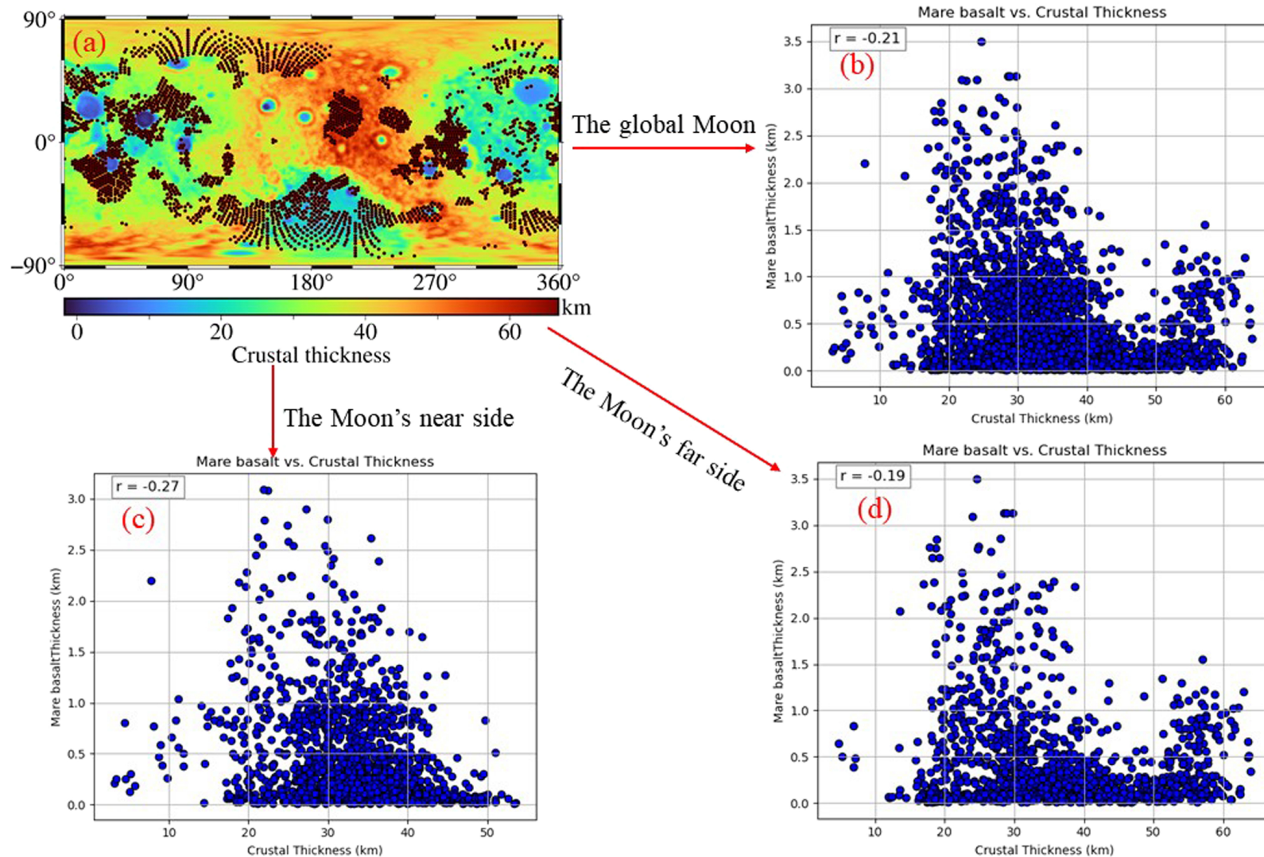
Figure 15. from Wensong Zhang et al 2026 Astron. J. 171 doi:10.3847/1538-3881/ae168d https://dx.doi.org/10.3847/1538-3881/ae168d © 2025. The Author(s). Published by the American Astronomical Society.
