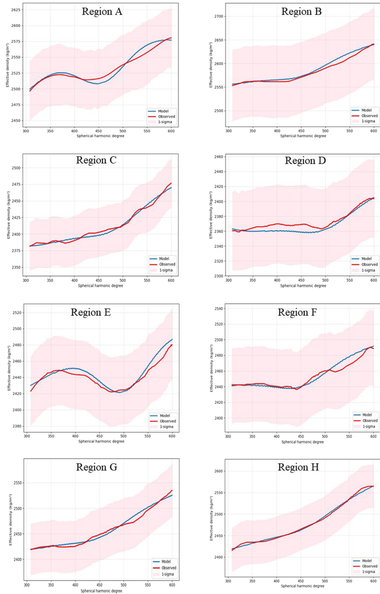
Figure 13. from Wensong Zhang et al 2026 Astron. J. 171 doi:10.3847/1538-3881/ae168d https://dx.doi.org/10.3847/1538-3881/ae168d © 2025. The Author(s). Published by the American Astronomical Society.
