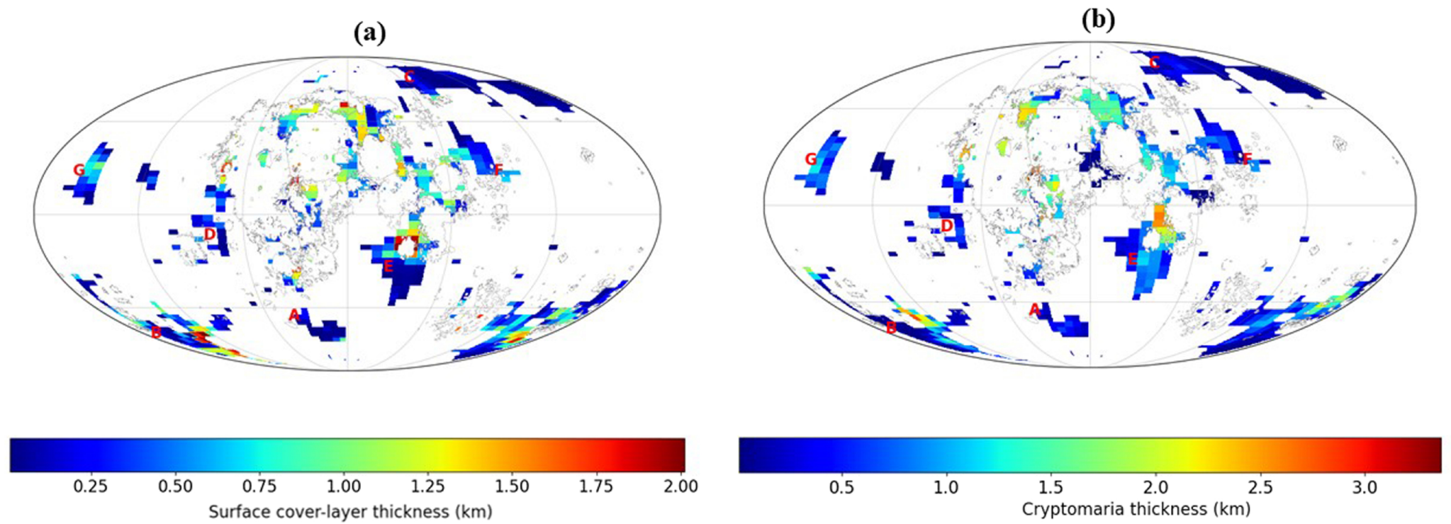
Figure 11. from Wensong Zhang et al 2026 Astron. J. 171 doi:10.3847/1538-3881/ae168d https://dx.doi.org/10.3847/1538-3881/ae168d © 2025. The Author(s). Published by the American Astronomical Society.
