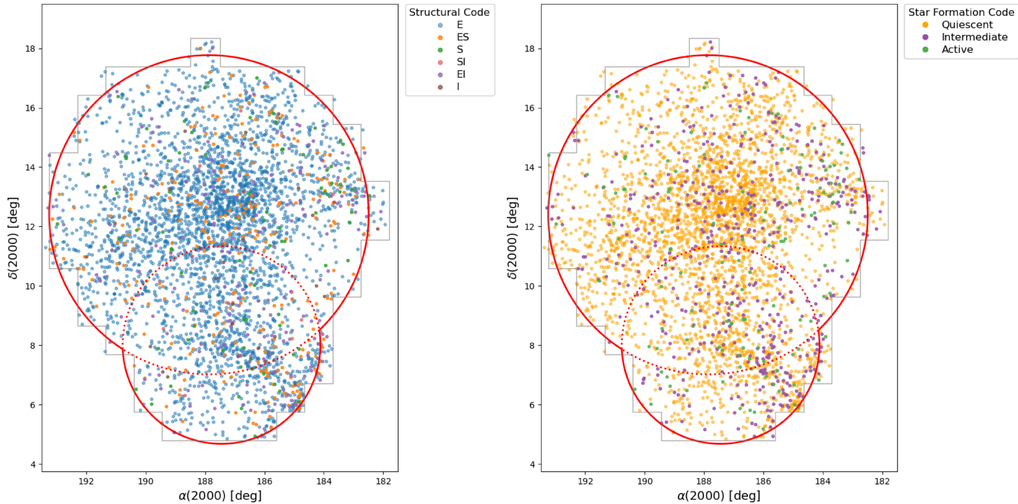
Figure 9. from Max M. Kurzner et al 2025 Astron. J. 170 doi:10.3847/1538-3881/ae1616 https://dx.doi.org/10.3847/1538-3881/ae1616 © 2025. The Author(s). Published by the American Astronomical Society.
