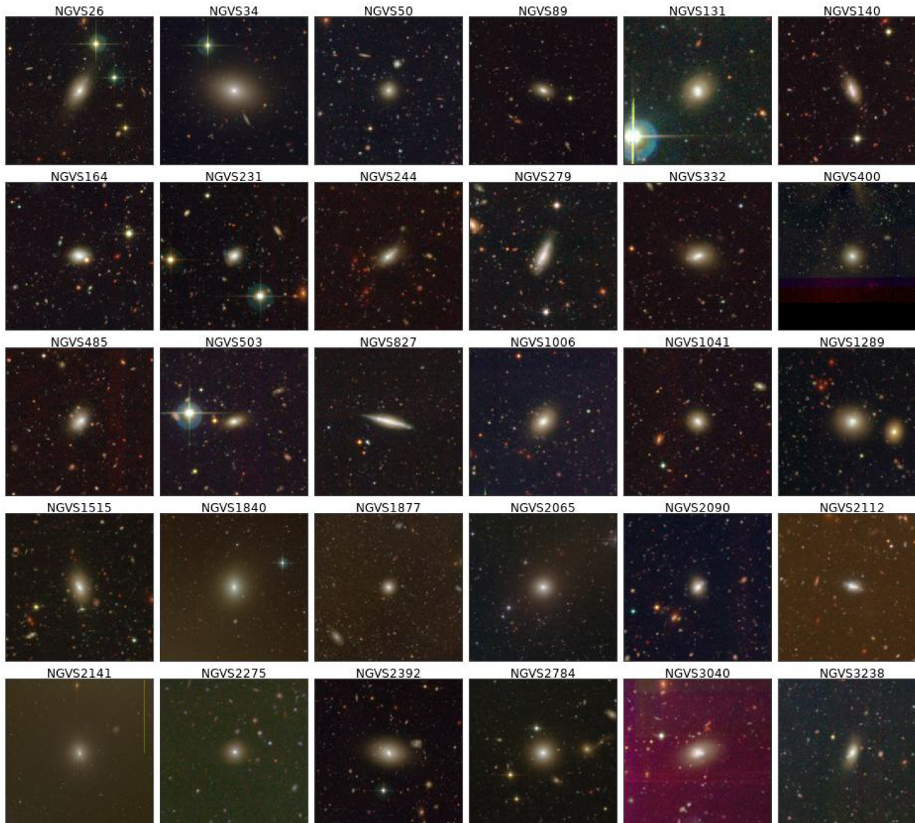
Figure 14. from Max M. Kurzner et al 2025 Astron. J. 170 doi:10.3847/1538-3881/ae1616 https://dx.doi.org/10.3847/1538-3881/ae1616 © 2025. The Author(s). Published by the American Astronomical Society.
