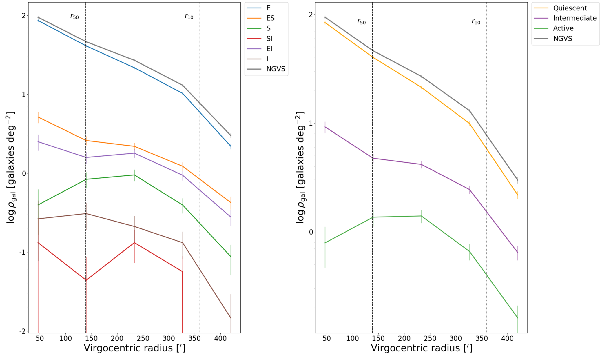
Figure 11. from Max M. Kurzner et al 2025 Astron. J. 170 doi:10.3847/1538-3881/ae1616 https://dx.doi.org/10.3847/1538-3881/ae1616 © 2025. The Author(s). Published by the American Astronomical Society.
