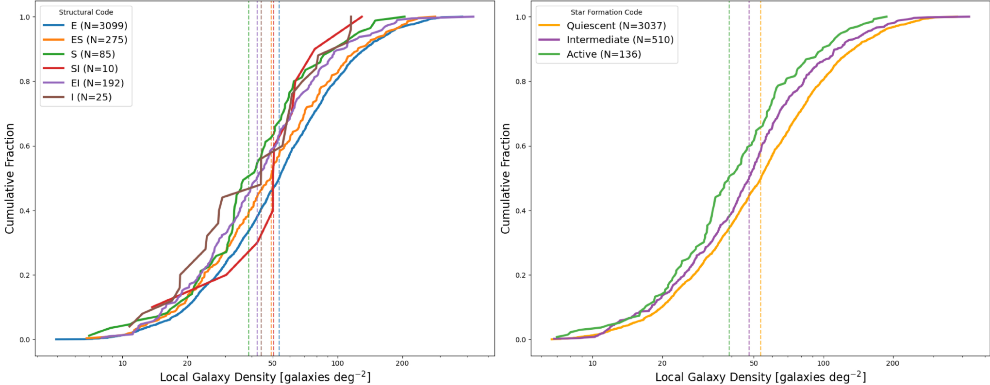
Figure 10. from Max M. Kurzner et al 2025 Astron. J. 170 doi:10.3847/1538-3881/ae1616 https://dx.doi.org/10.3847/1538-3881/ae1616 © 2025. The Author(s). Published by the American Astronomical Society.
